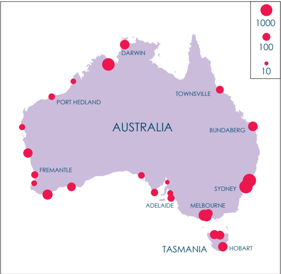
Figure 39: Projected increase in frequency of flooding events from the sea for a sea-level rise of 0.5 m.
