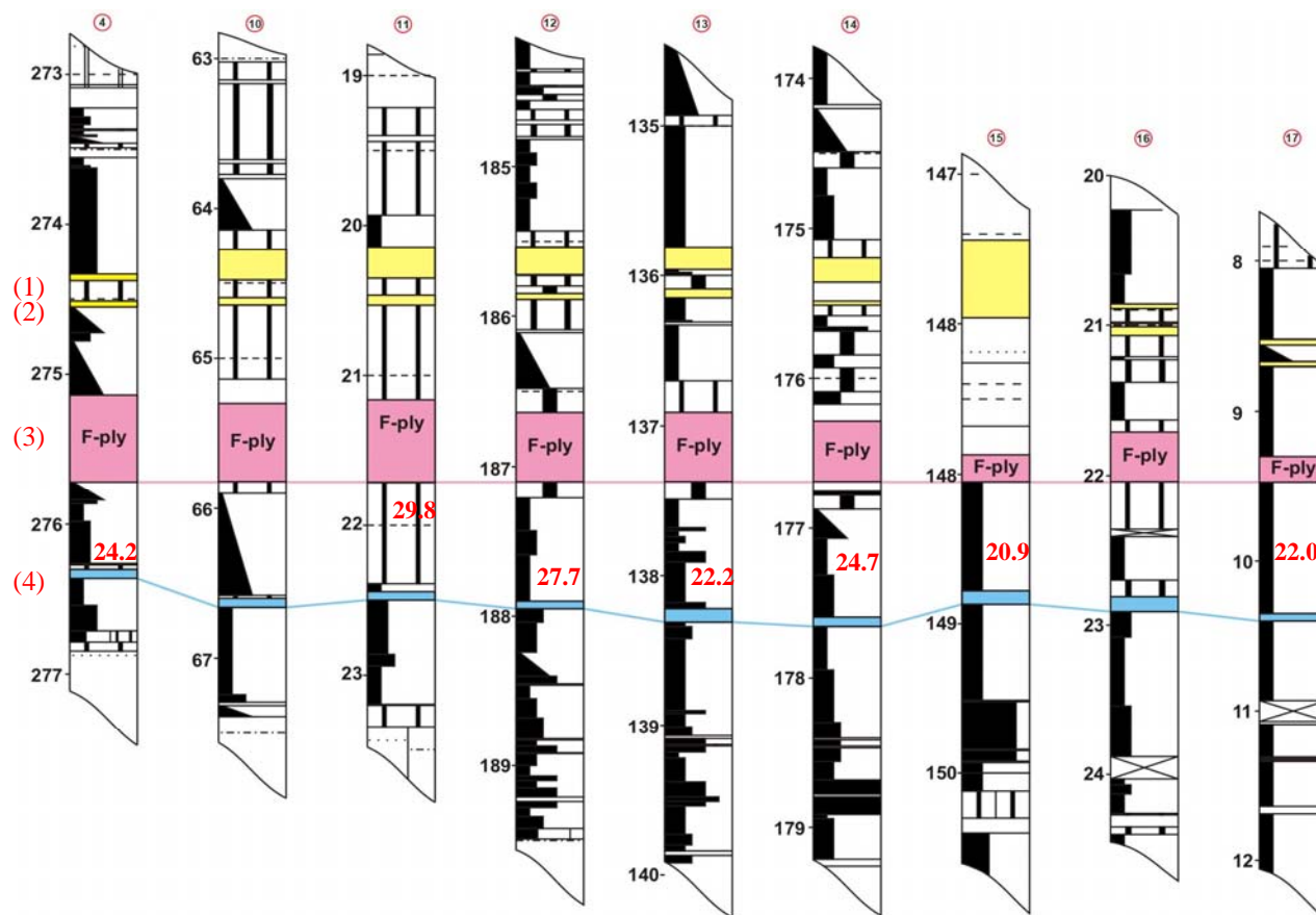
Figure 5 North-south cross-section from Bylong to Ivanhoe North, Lidsdale Coal (for location of boreholes see Figure 1)
