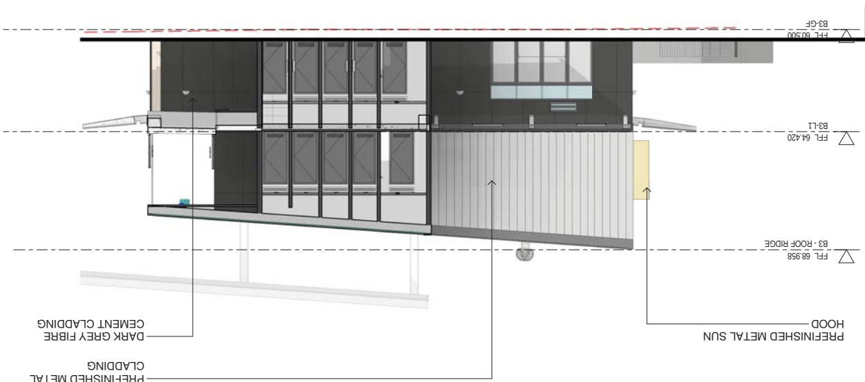
1 B3 WEST ELEVATION 1 : 100
