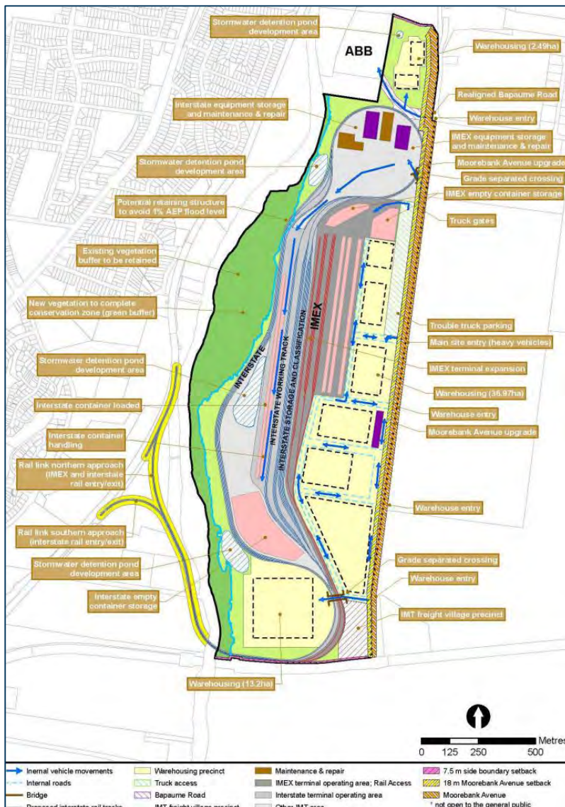
Figure 4-3 Proposed MIC Site Layout
