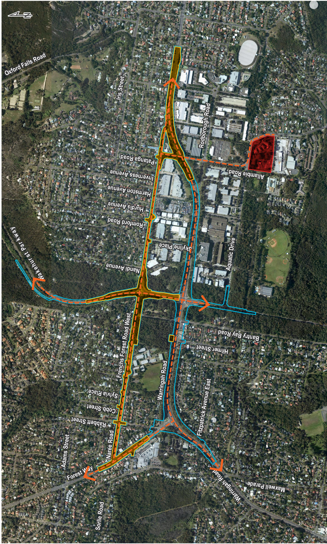
Stage 1 haulage routes Figure 5-10
