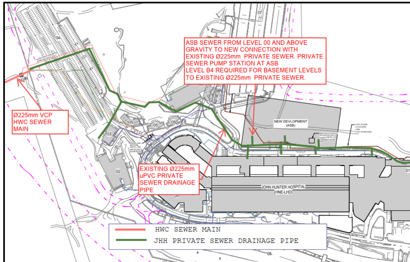
Figure 2-2: Existing Hunter Water Corporation sewer main surrounding the site (Based on surveys and DBYD)
