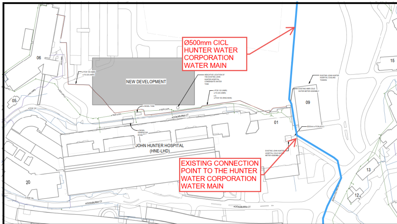
Figure 2-5: Existing Hunter Water Corporation water main surrounding the site (Based on surveys and DBYD)
