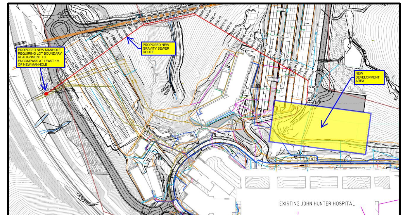
Figure 2-3 Proposed Gravity Sewer Main Option Route Plan
