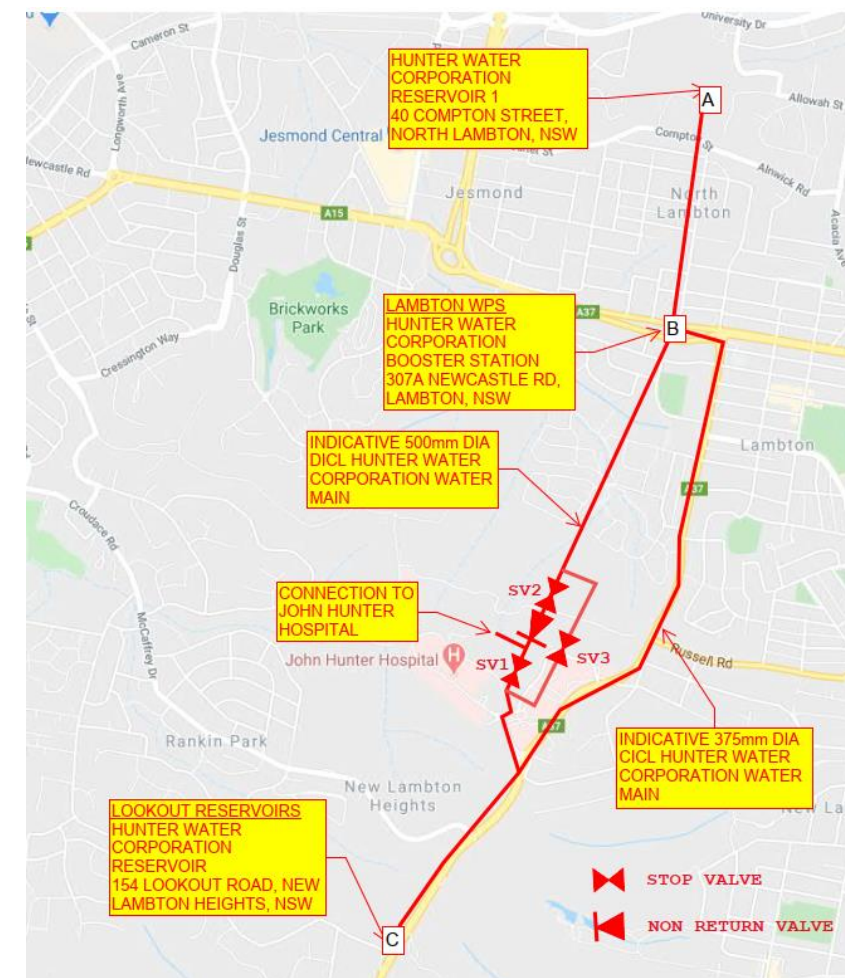
Figure 2-6: Indicative sketch showing the Hunter Water Corporation water main around John Hunter Hospital
