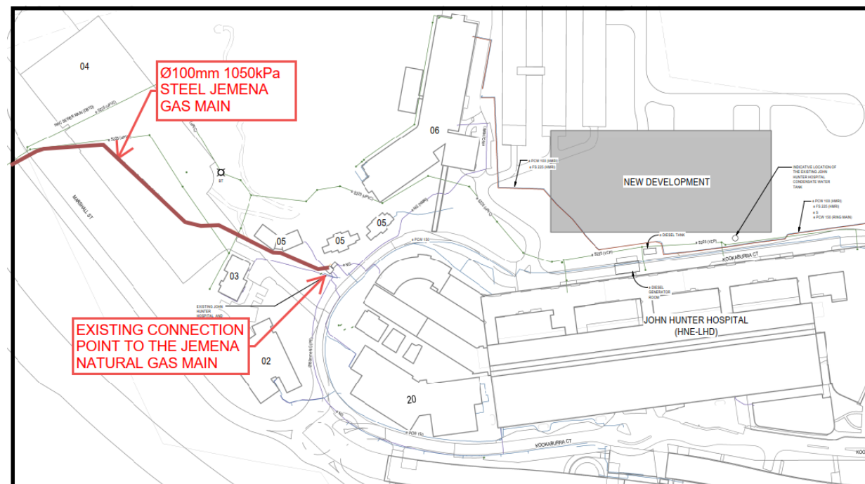
Figure 2-8: Existing Jemena Gas main surrounding the site (Based on surveys and DBYD)
