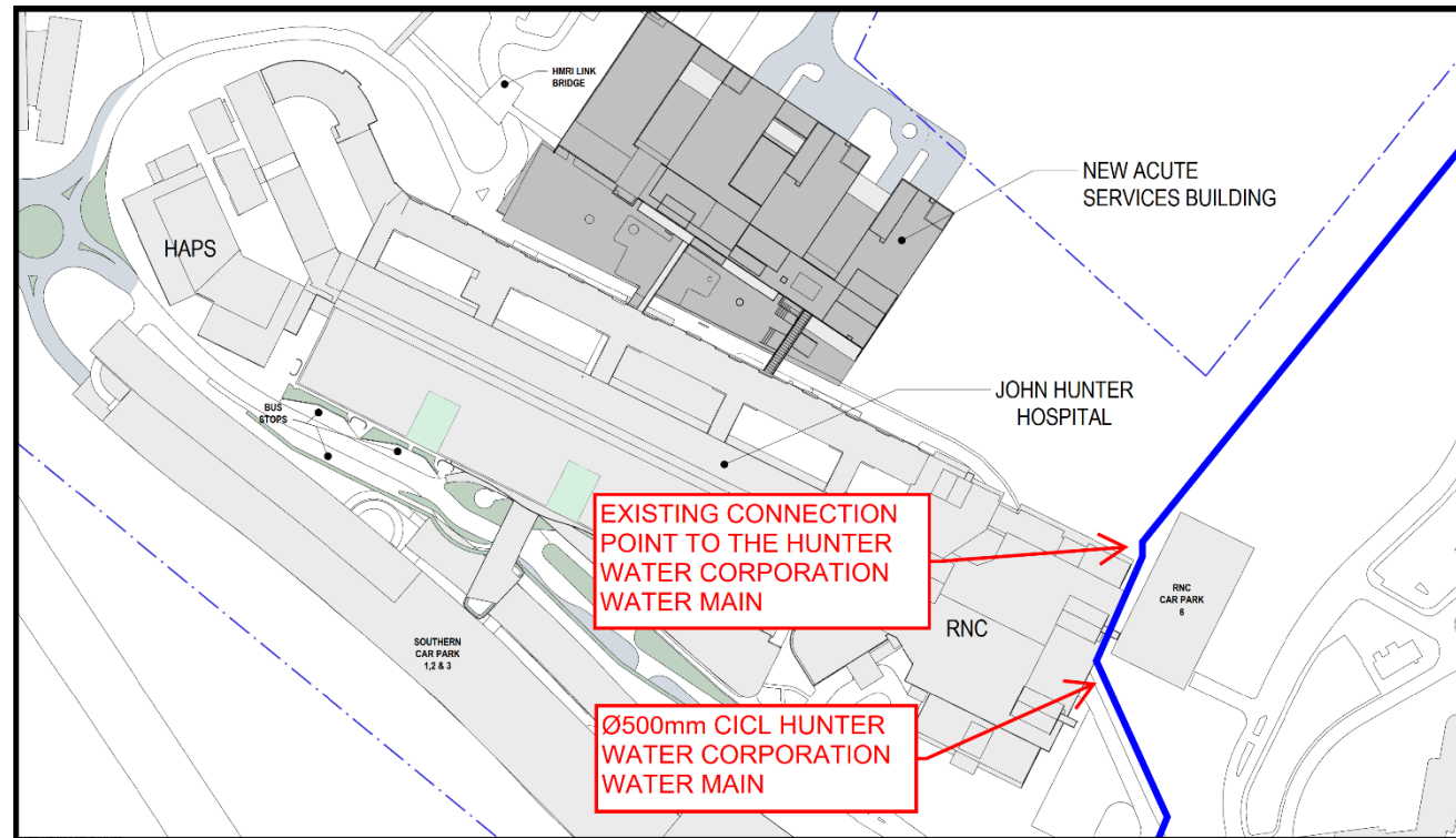
Figure 2-7: Existing Hunter Water Corporation water main surrounding the site (Based on surveys and DBYD)
