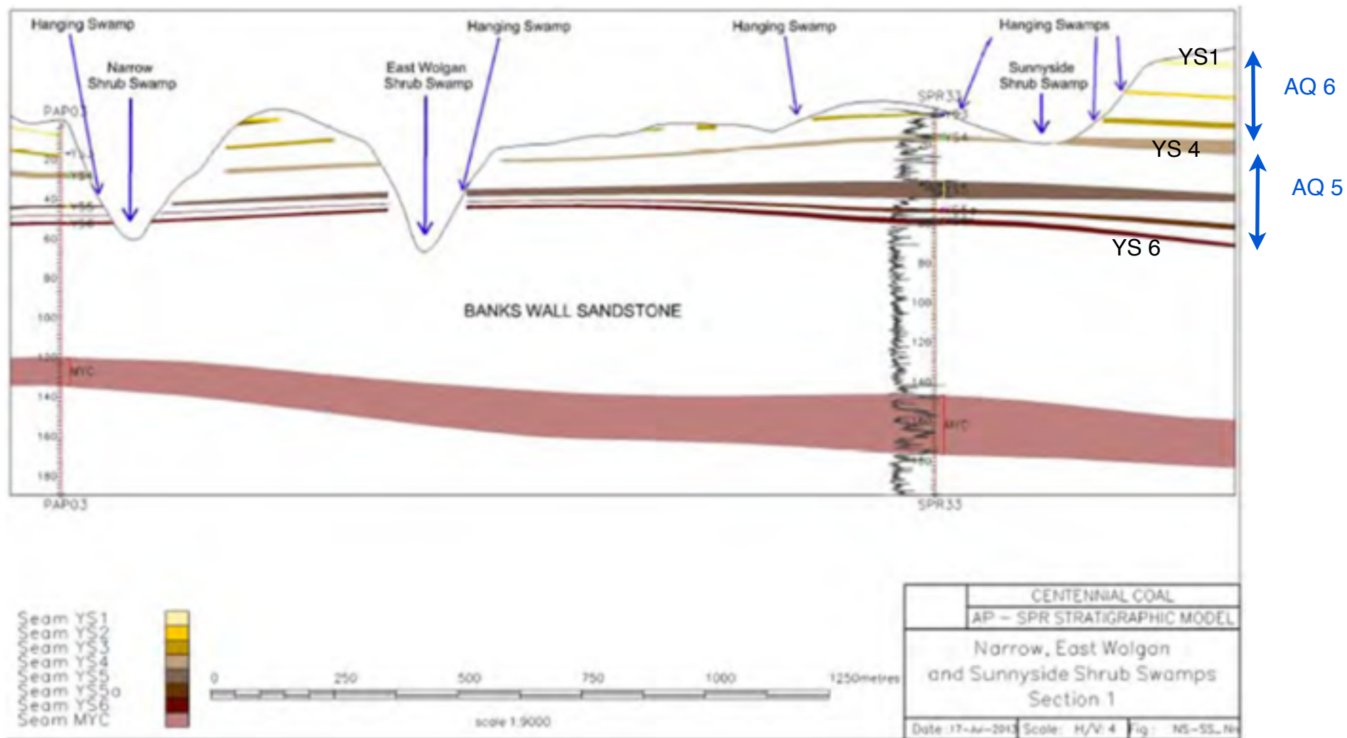
Figure 2.10 Cross Section through Geology and Topography of Narrow Swamp, East Wollan Swamp and Sunnyside Swamp
