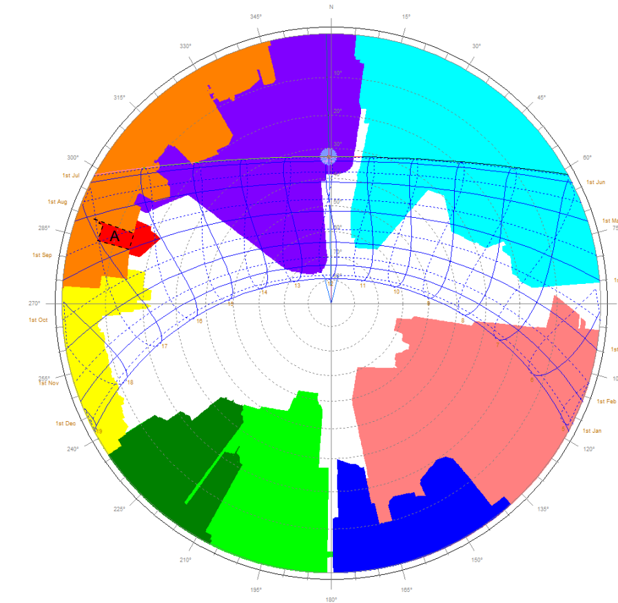
sky map 2 north east corner exposure dates: 03 Sep - 23 Sep / 22 Mar - 15 Apr
