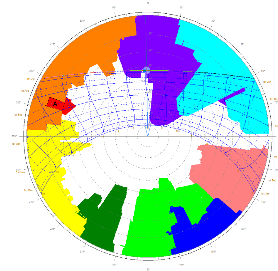
sky map 1 north west corner exposure dates: 01 Sep - 21 Sep / 21 Mar - 14 Apr
