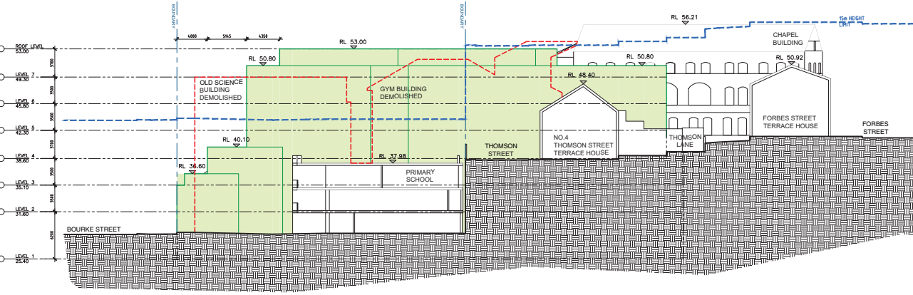
SECTION FF
