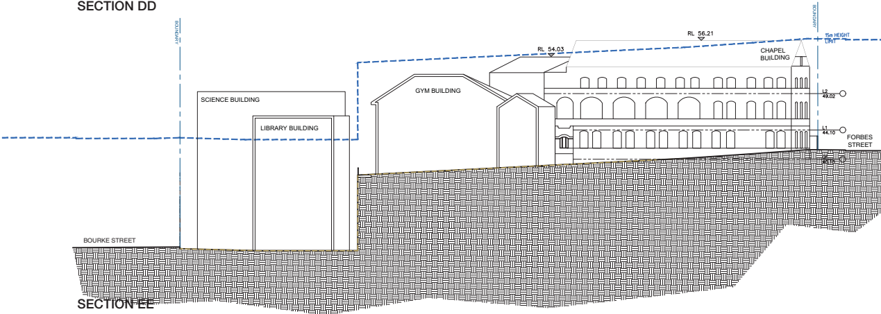
SECTION EE
