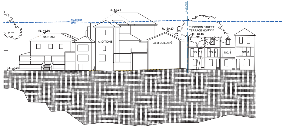
SECTION GG
