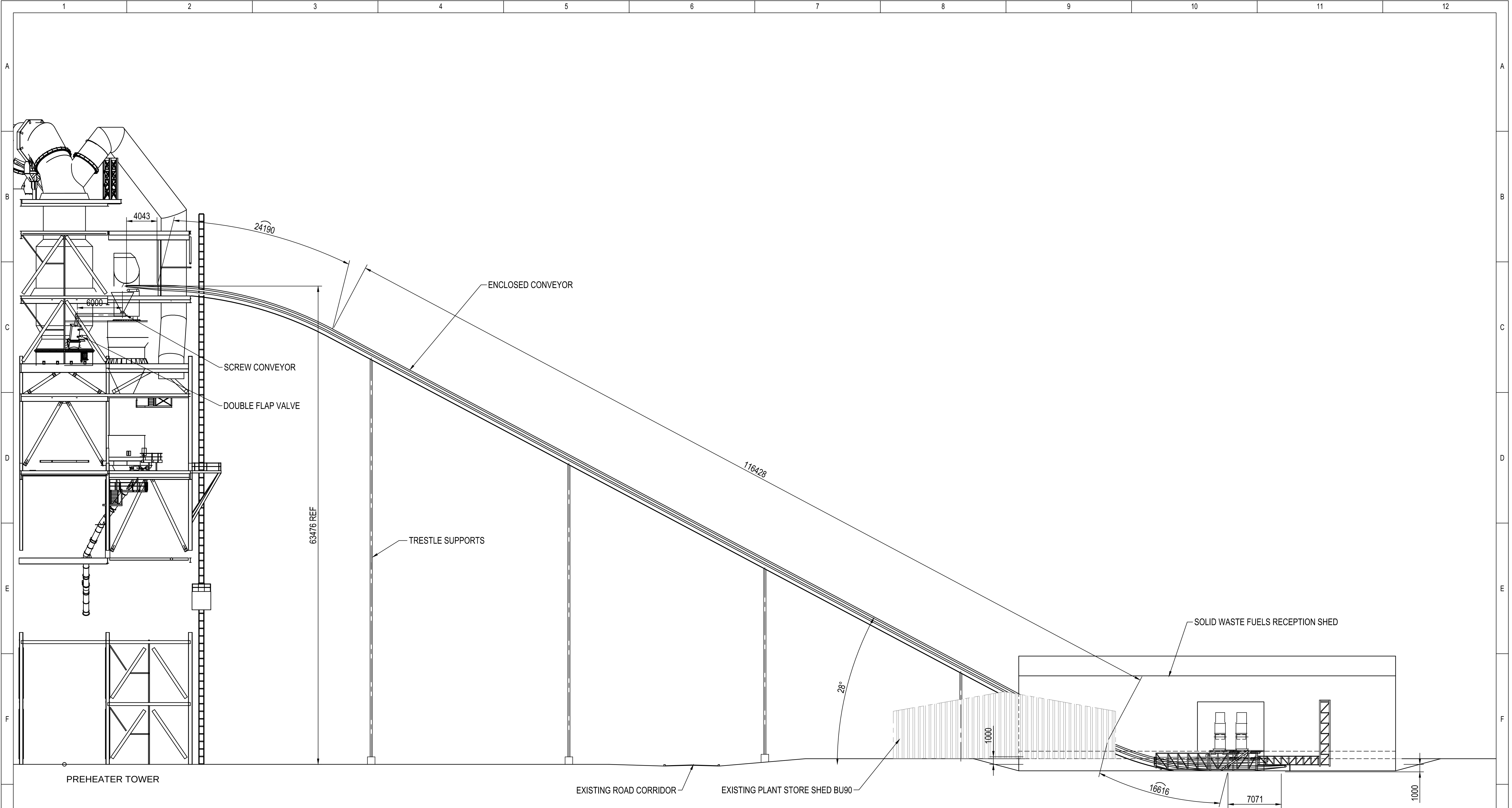
ELEVATION LOOKING WEST
