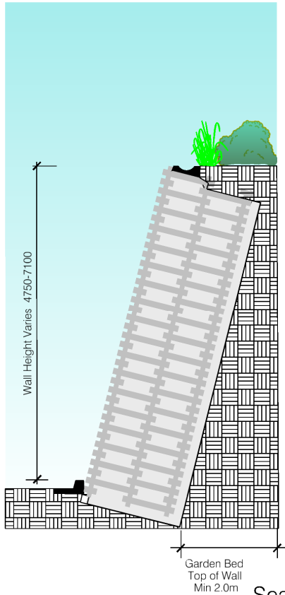
A Retaining Wall and Garden Detail Scale 1:50 @ A1
