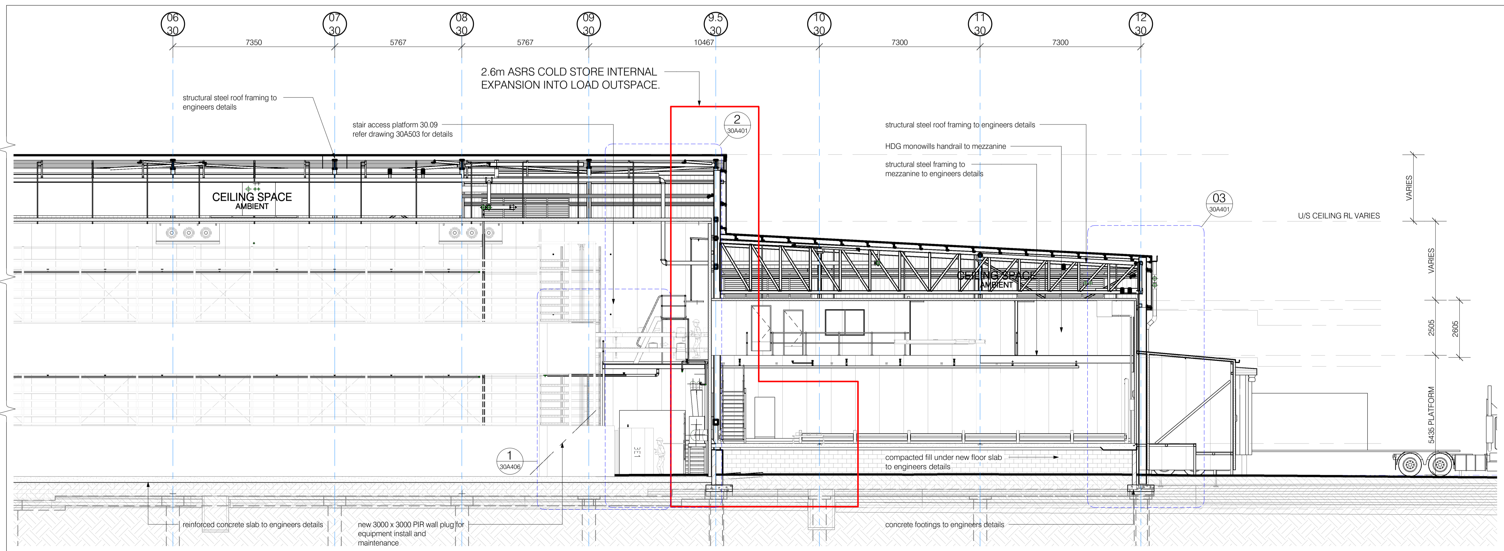
02 30A103 SECTION - EAST END A1 = 1 : 100
