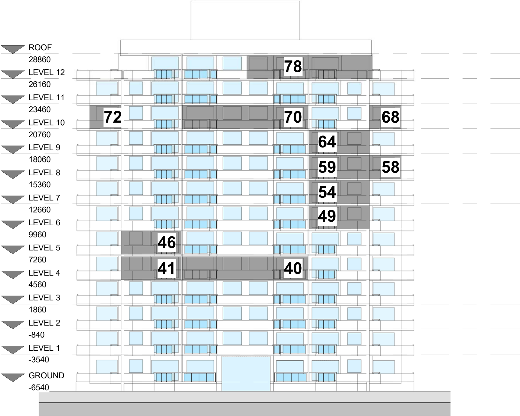
NORTH ELEVATION
