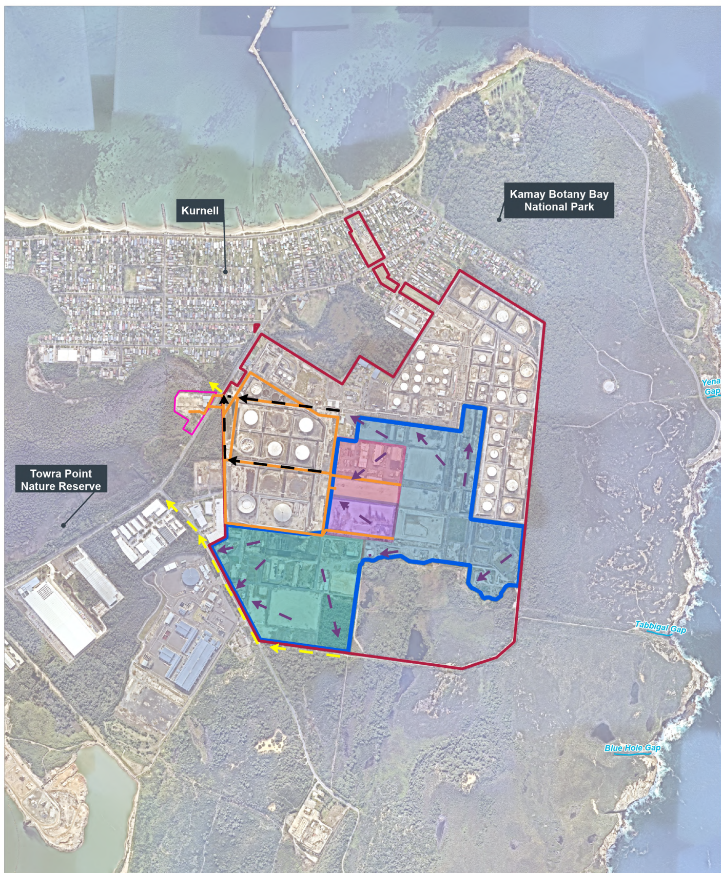
FIGURE 3-3. CONCEPT STORMWATER STRATEGY
