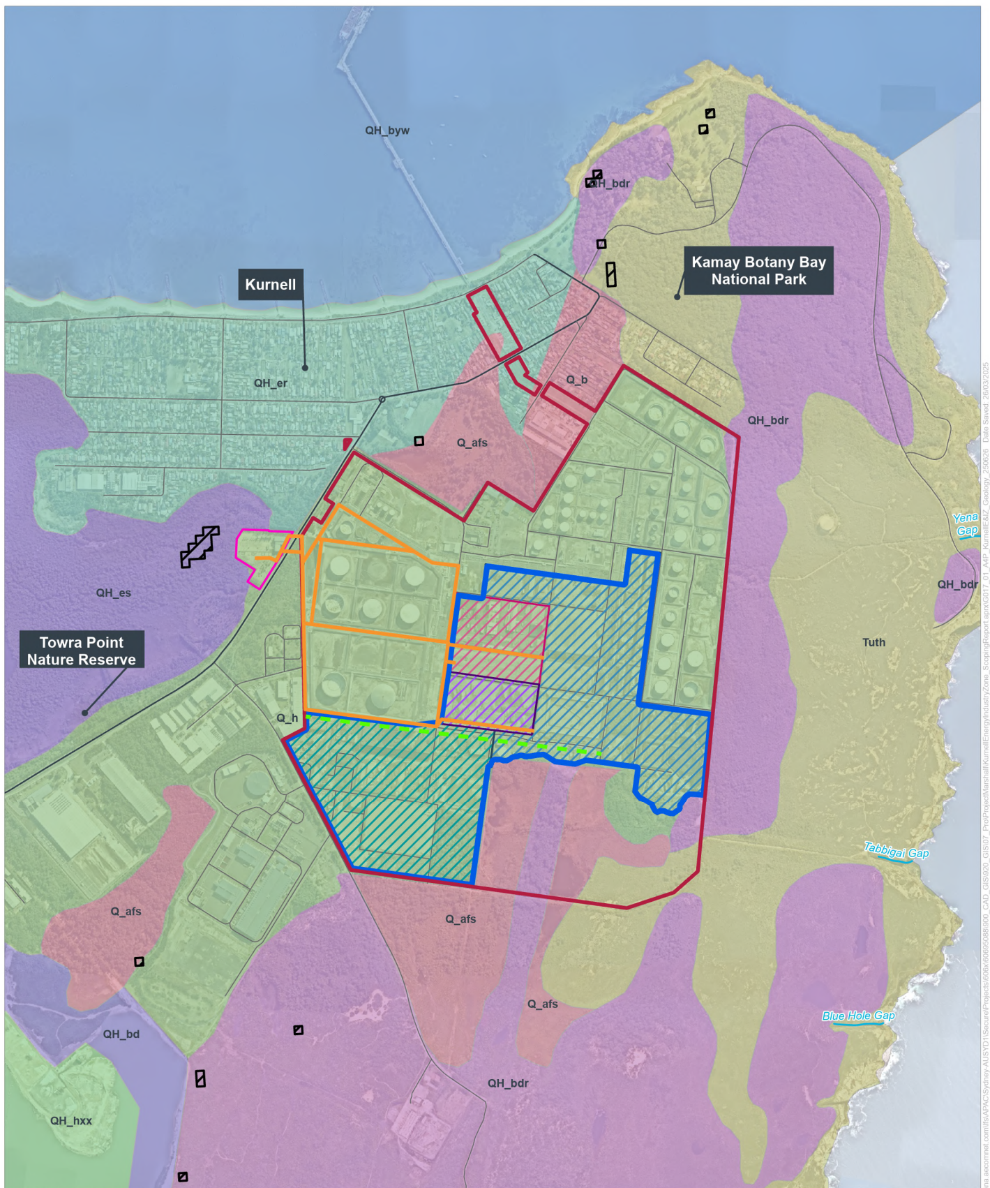
FIGURE 6-1. GEOLOGY
