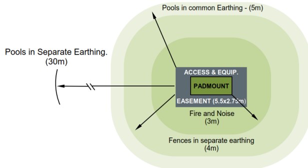
A4.3 - Padmount easements and clearances
