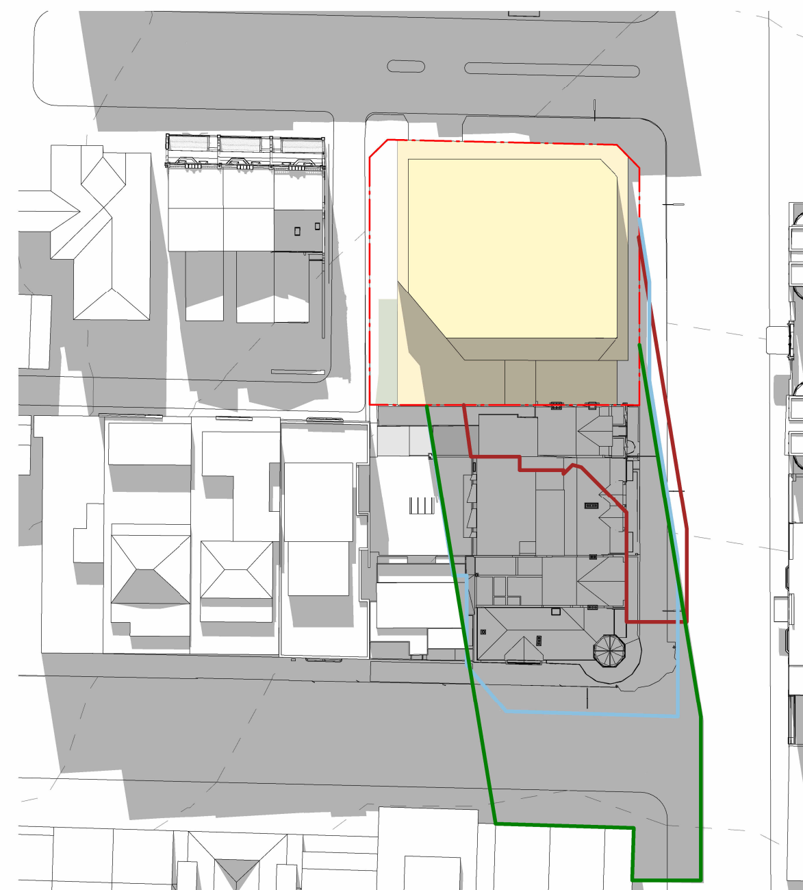
4 ENVELOPE - SHADOWS - 12pm 1 : 700
