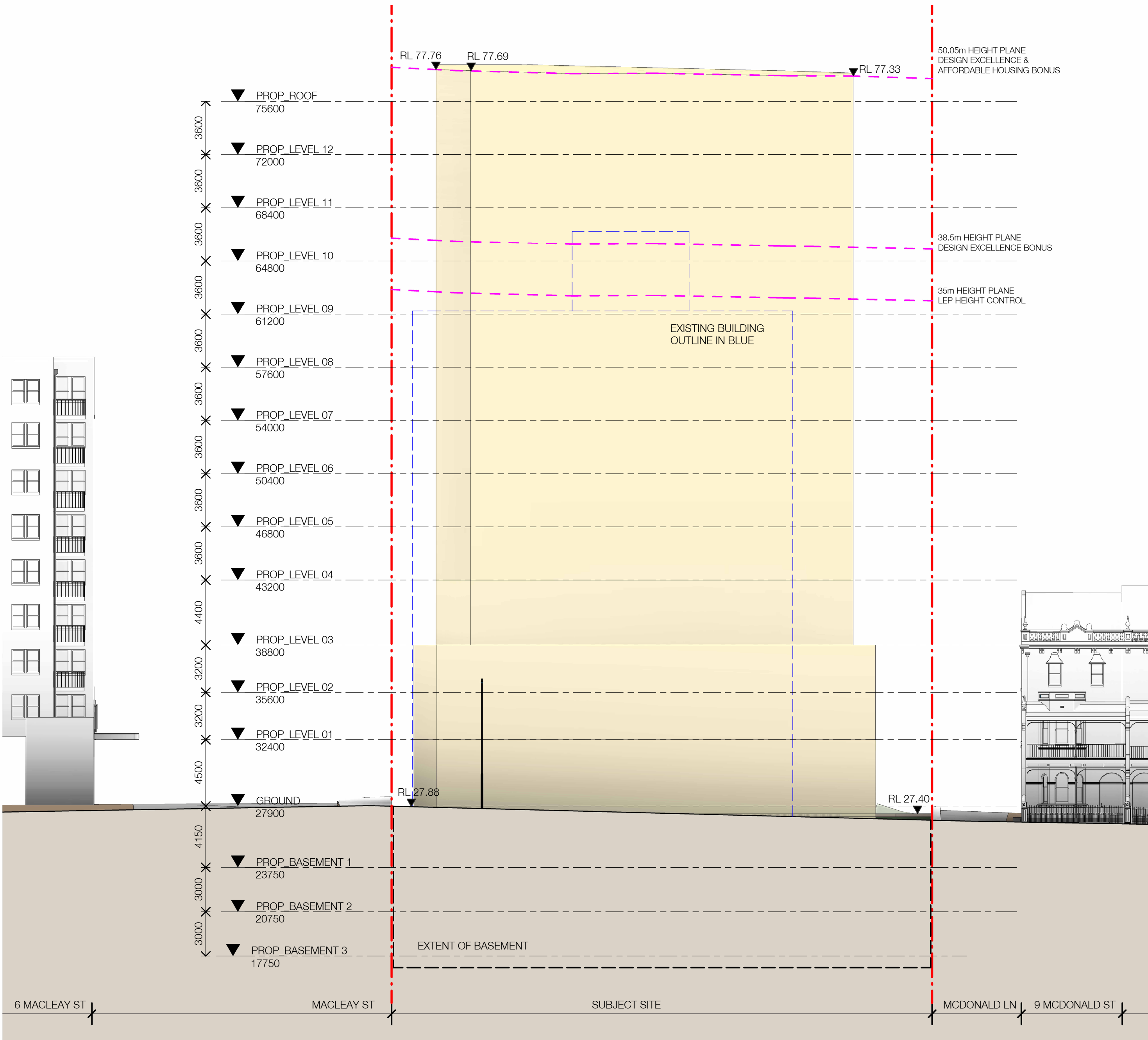
1 ENVELOPE - ELEVATION_NORTH 1 : 200
