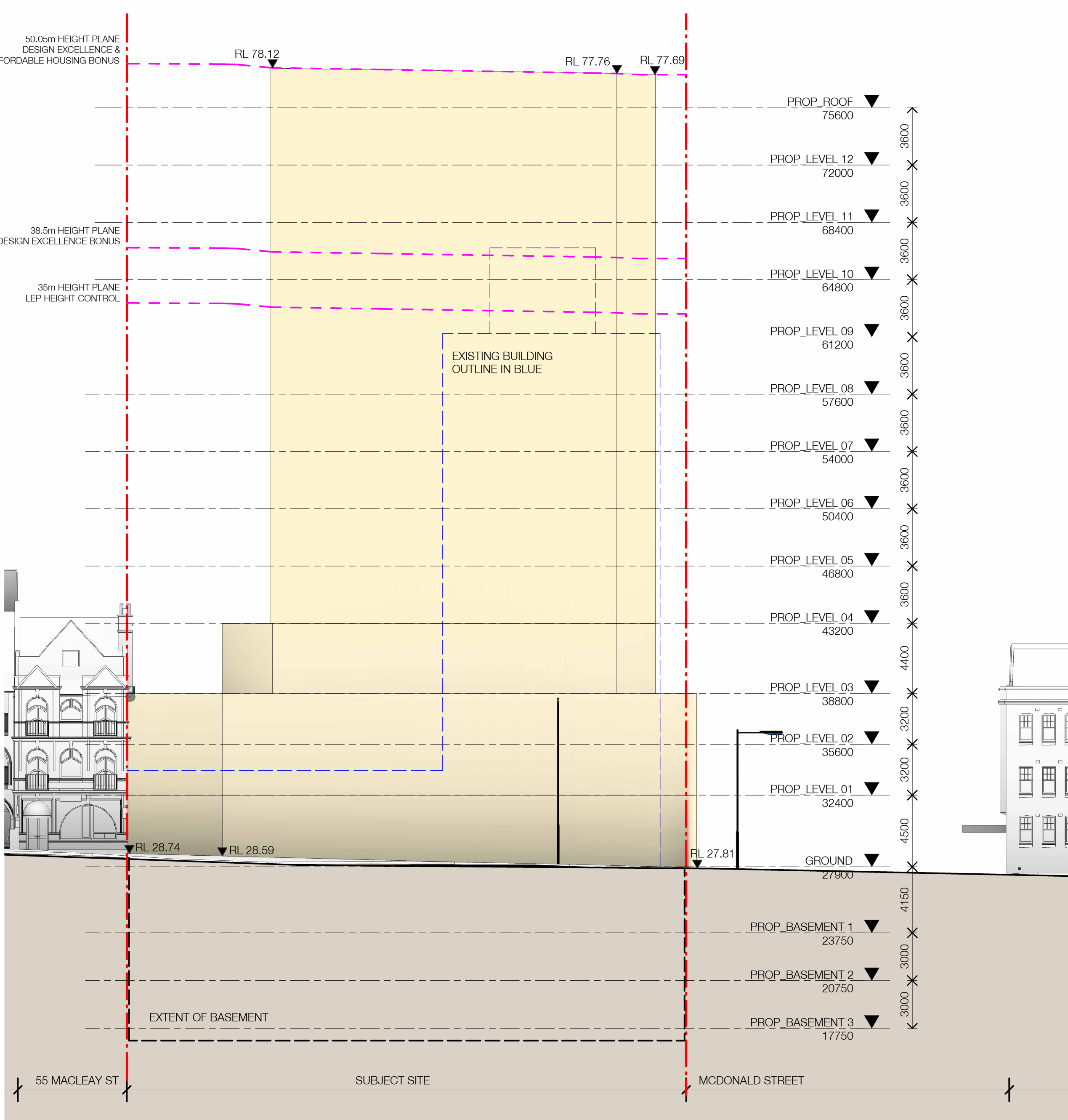
2 ENVELOPE - ELEVATION_EAST 1 : 200
