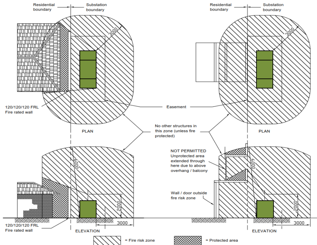
Figure 47 - Typical effect of screen walls
