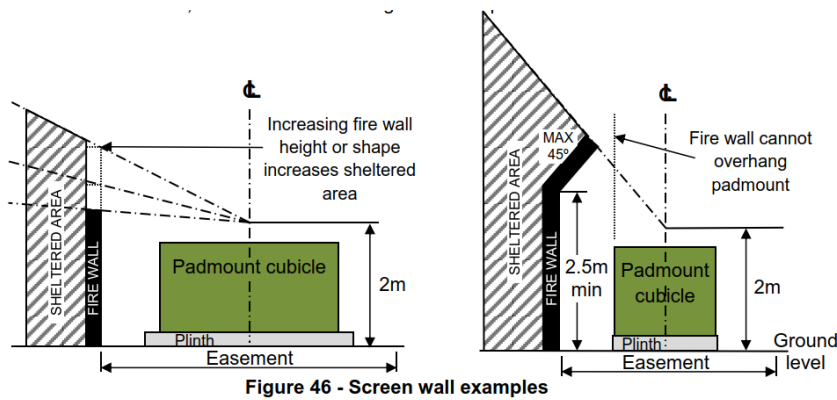
Figure 46 - Screen wall examples
