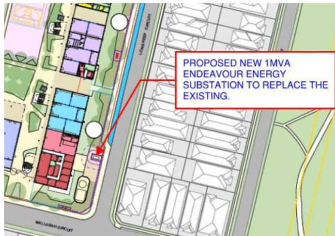
Figure E1: Electrical Infrastructure Site Plan
