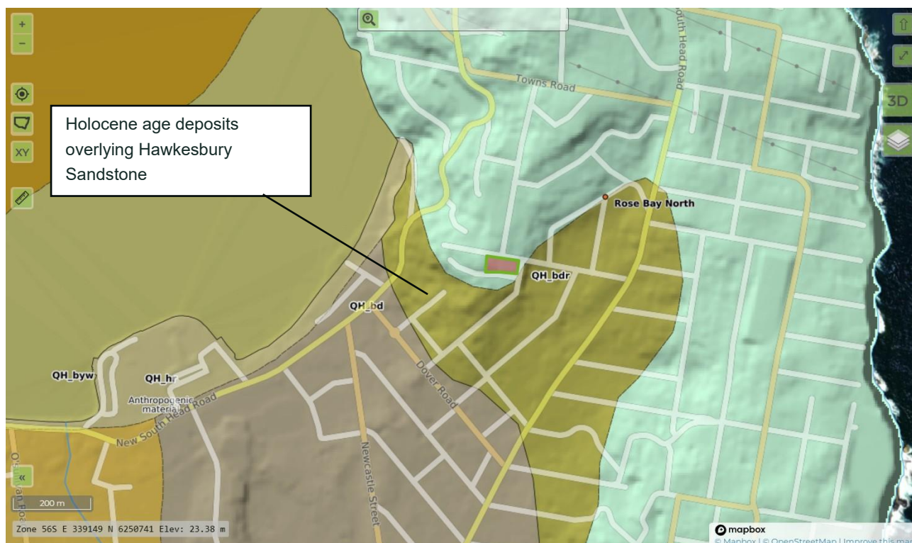
Plate 2-2: Extract of the Minview Seamless Geology Map Showing the vicinity of the site to be covered by Holocene age Coastal & Estuarine Deposits
