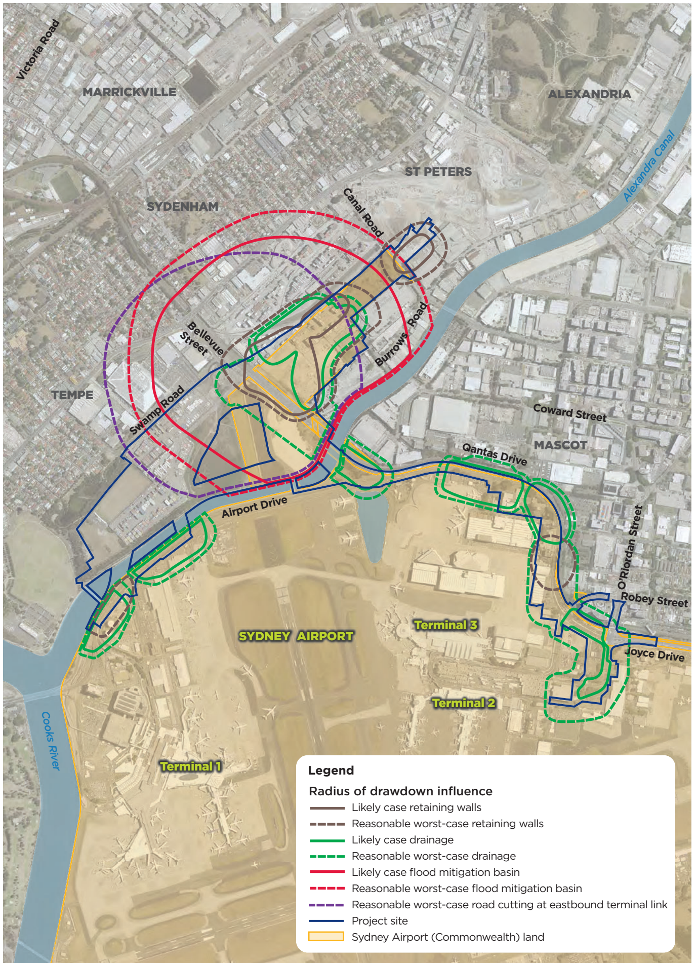
Figure 15.4 Radii of groundwater influence during construction
