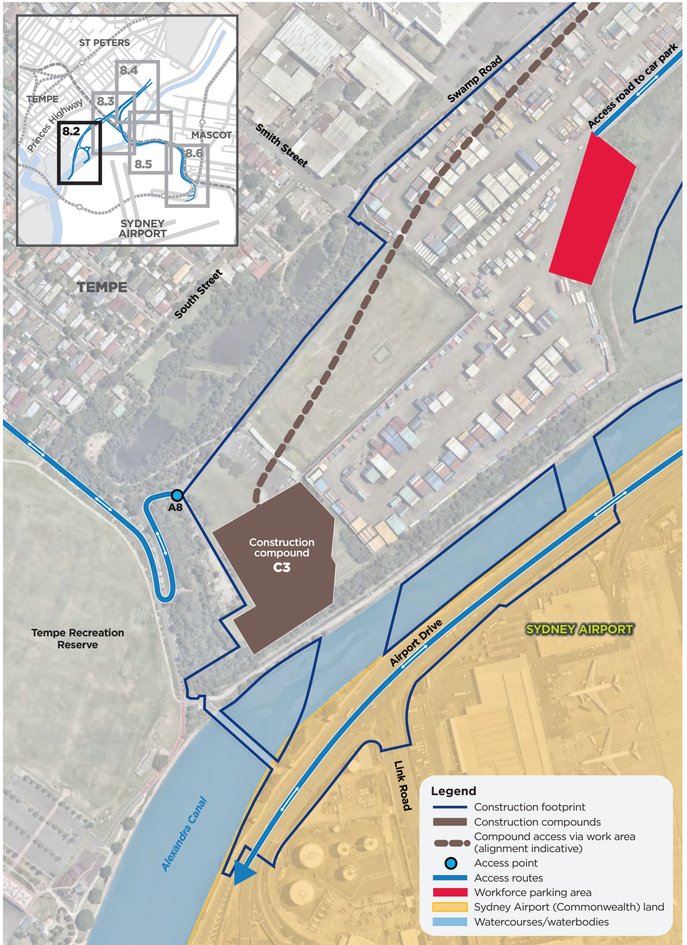
Figure 8.2 Construction footprint, work areas and facilities - map 1
