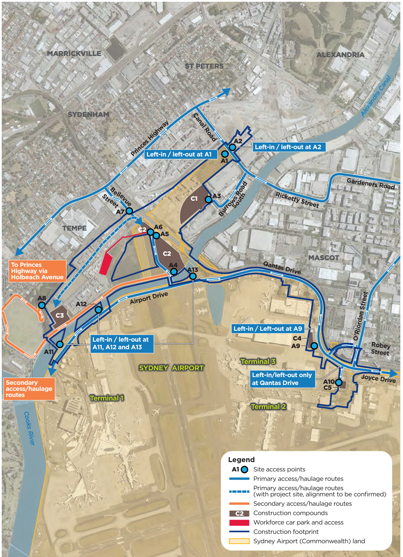
Figure 8.19 Preliminary site accesses and haulage routes
