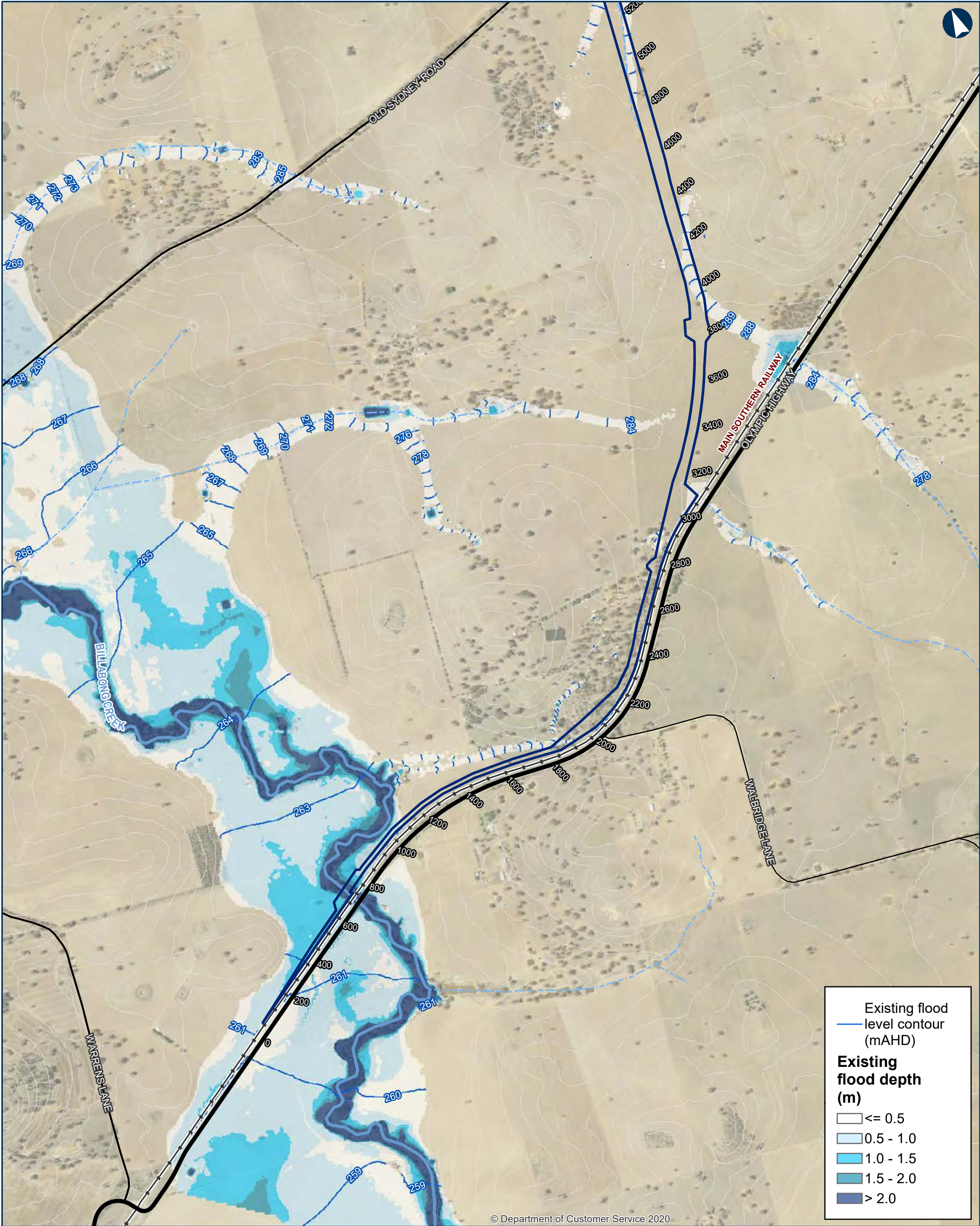
ILLABO TO STOCKINBINGAL 1% AEP Existing Flood Depths and Levels
