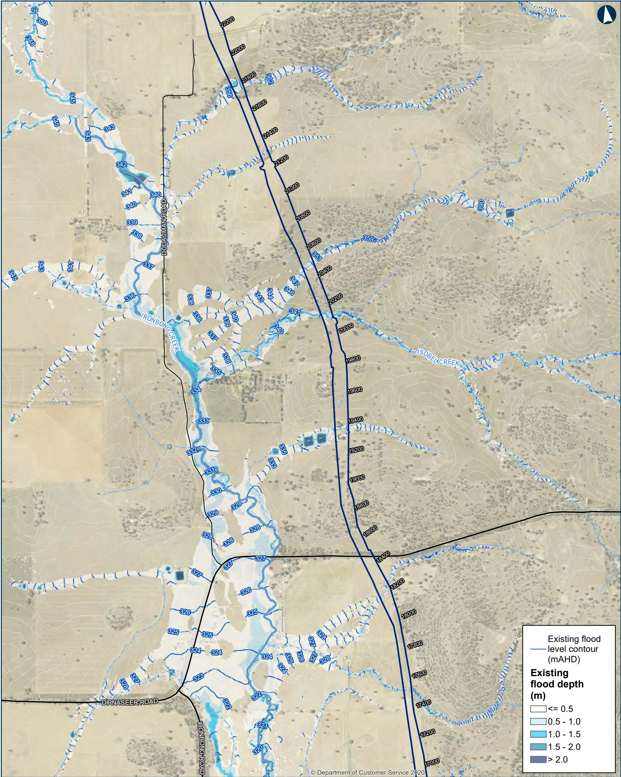
ILLABO TO STOCKINBINGAL 1% AEP Existing Flood Depths and Levels Map 5 of 9
