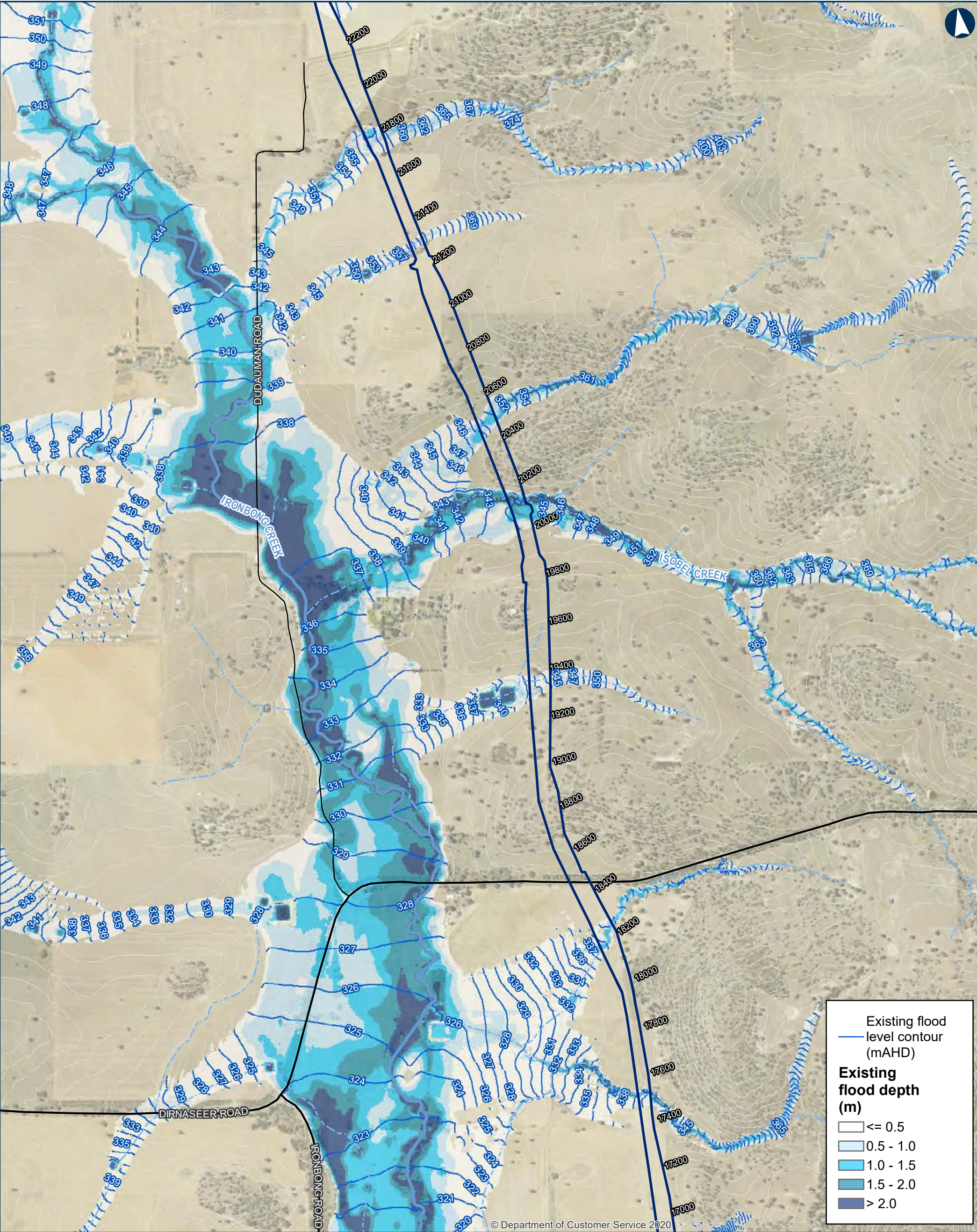
ILLABO TO STOCKINBINGAL Probable Maximum Flood Existing Flood Depths and Levels Map 5 of 9
