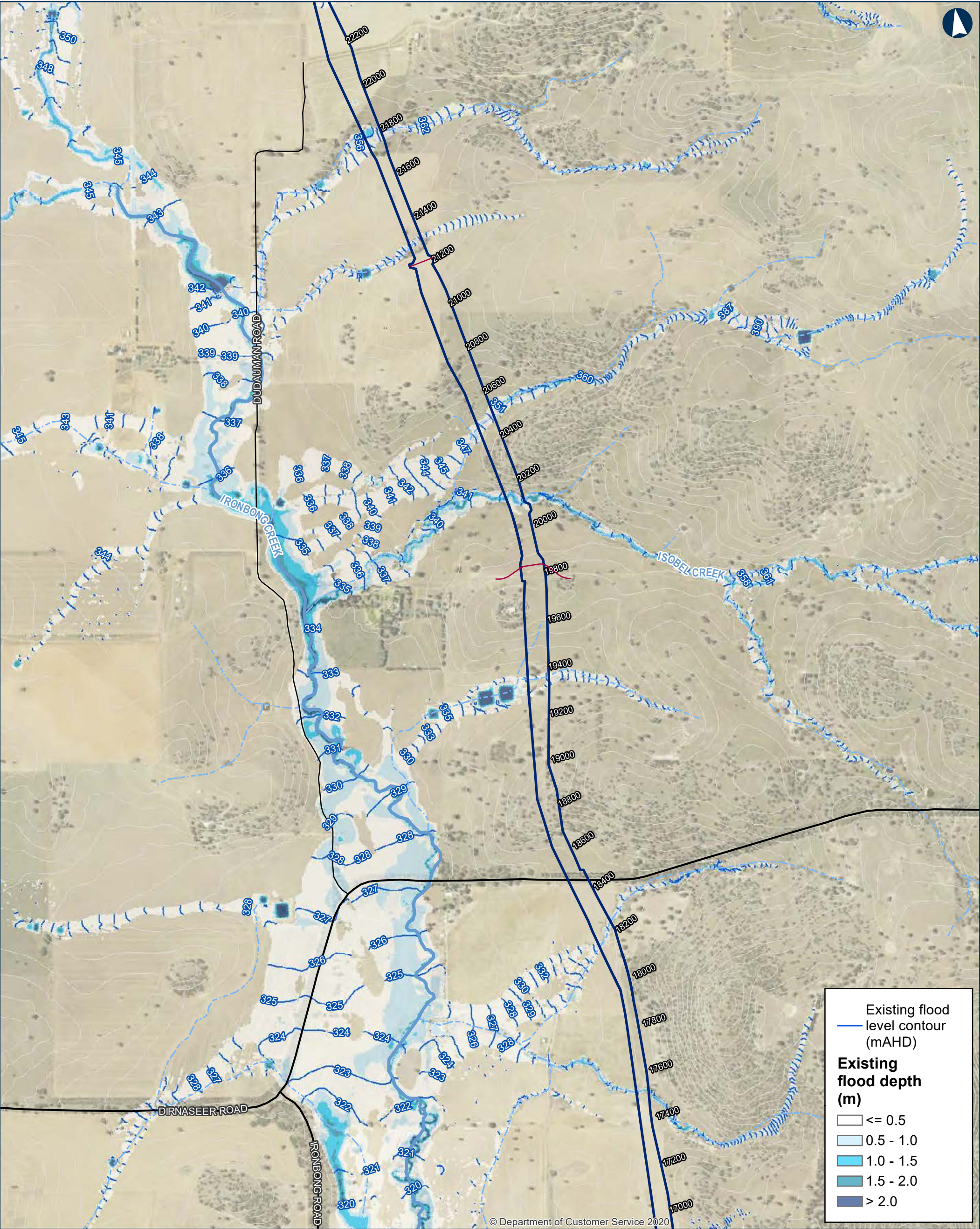
ILLABO TO STOCKINBINGAL 1% AEP Climate Change Existing Flood Depths and Levels Map 5 of 9
