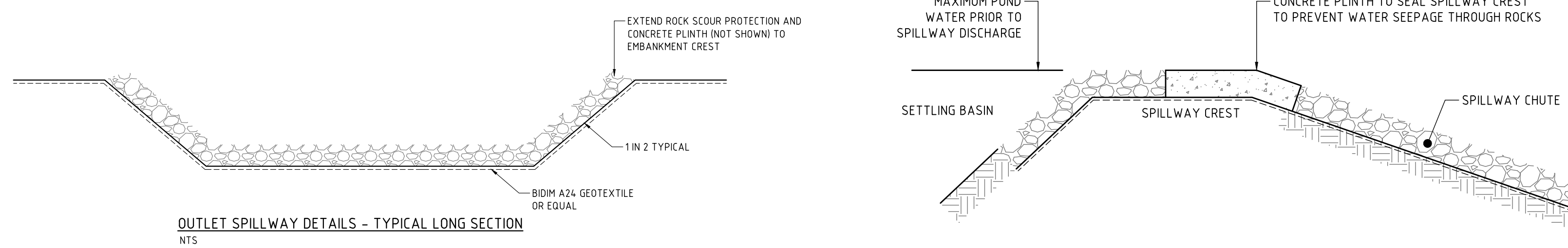
OUTLET SPILLWAY DETAILS - TYPICAL CROSS SECTION NTS
