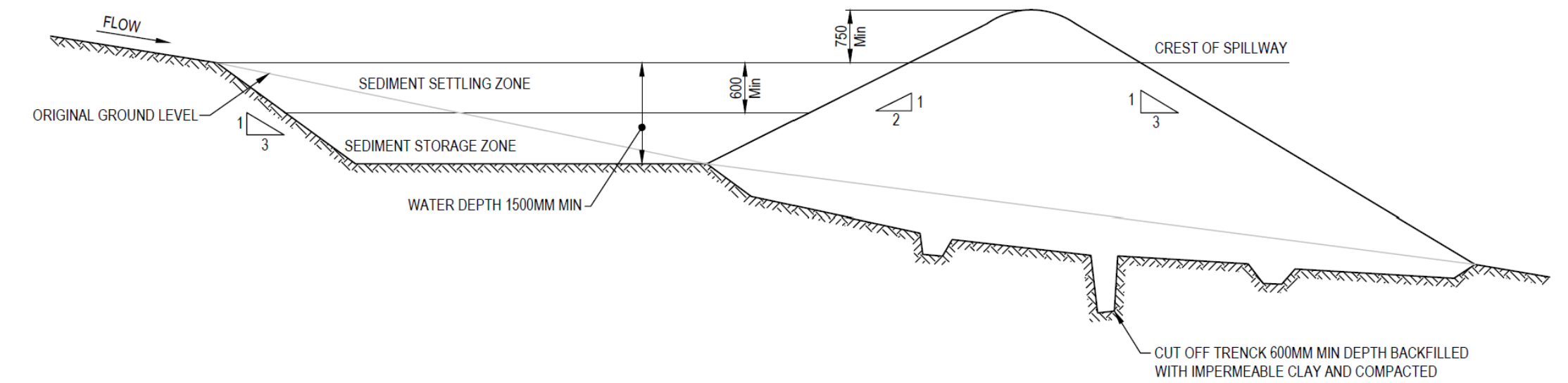
TYPICAL EARTH SEDIMENT BASIN DETAIL N.T.S
