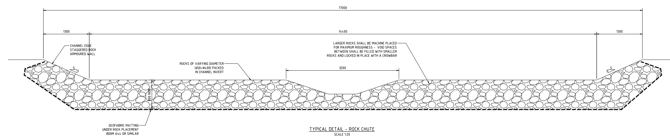
TYPICAL ROCK CHUTE / ROCK DRAIN
