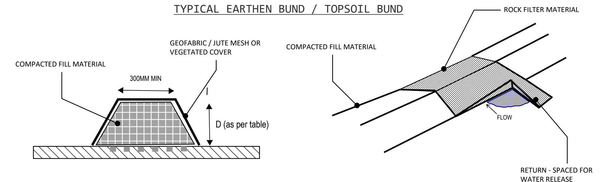
TYPICAL EARTHEN BUND / TOPSOIL BUND
