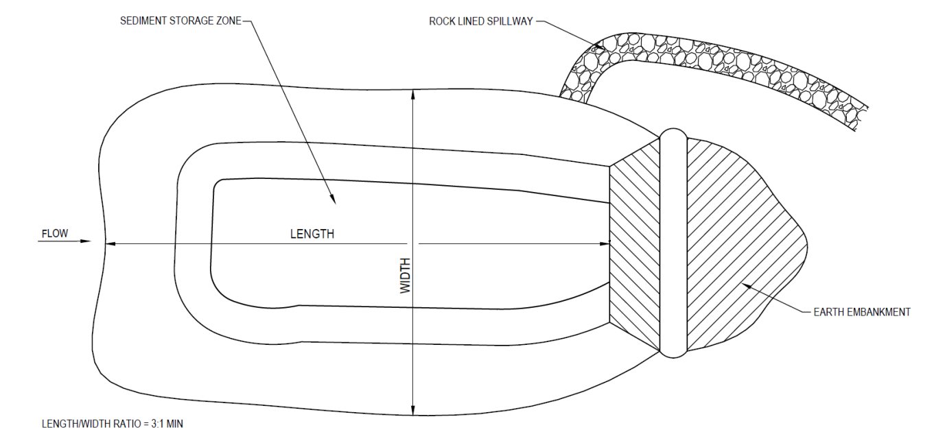
TYPICAL EARTH SEDIMENT BASIN DETAIL N.T.S
