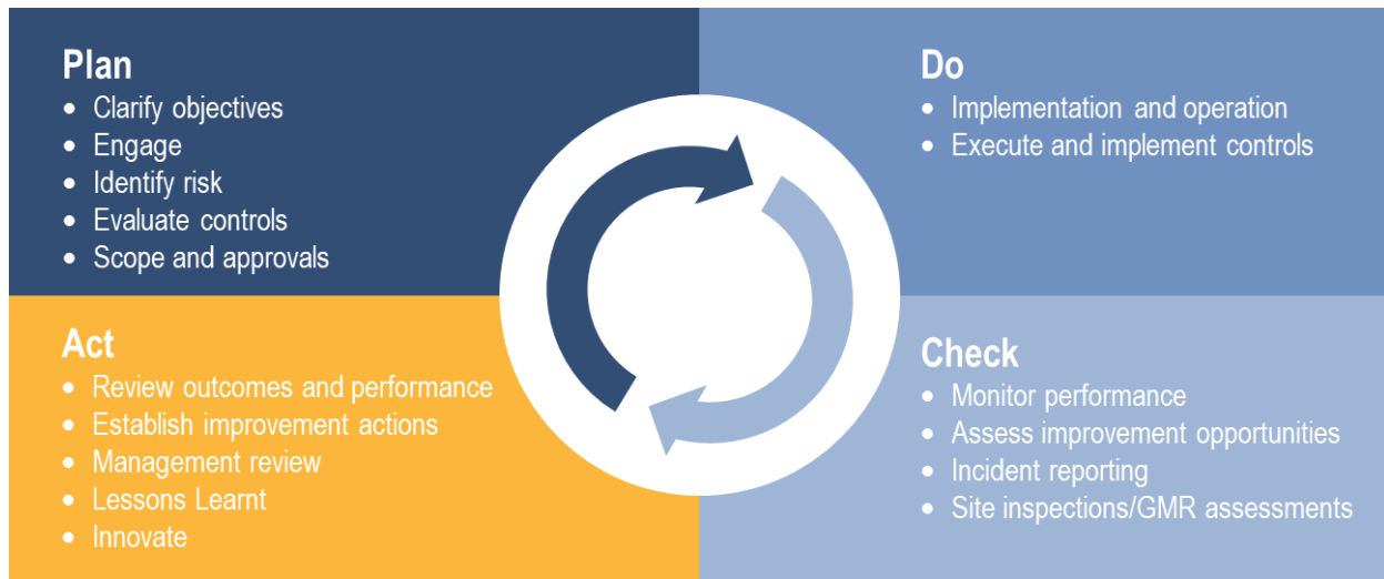
Figure 3-2 PDCA model
