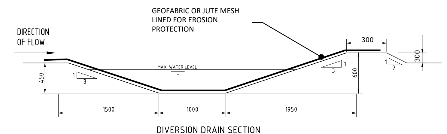
TYPICAL DIVERSION DRAIN
