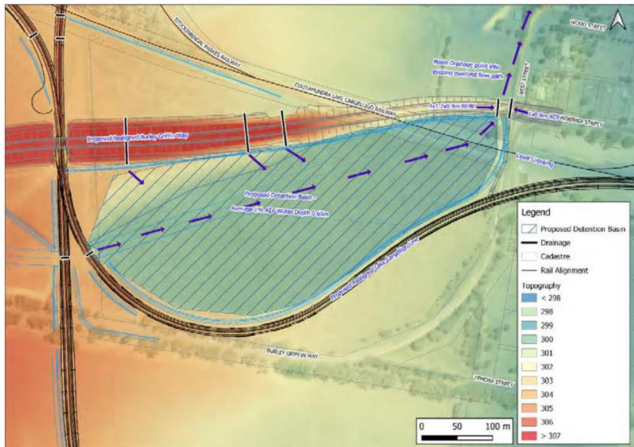
Figure 4-3 - Detention Basin near Burley Griffin Way
