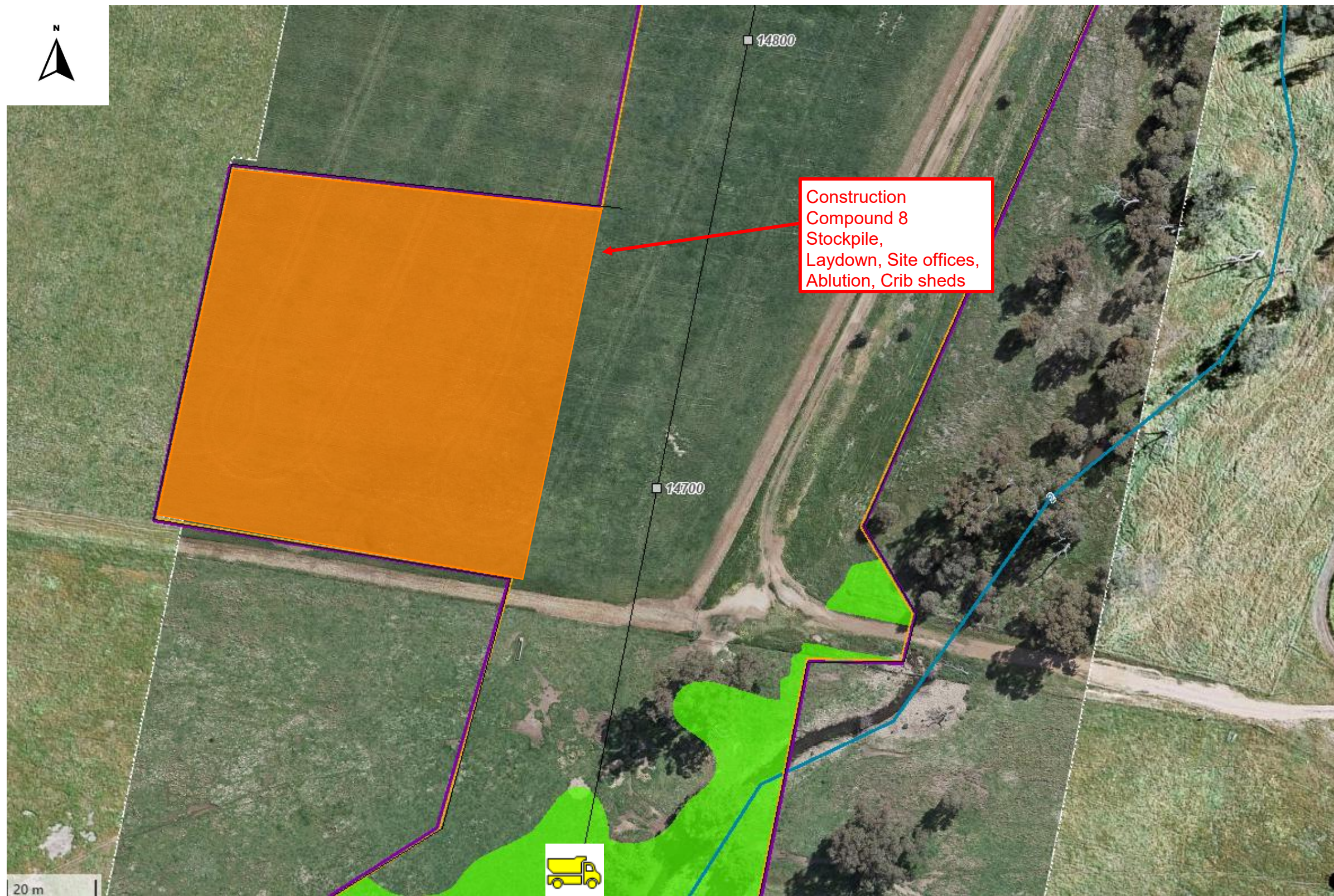
ILLABO TO STOCKINBINGAL Figure A8-8 Site Compounds
