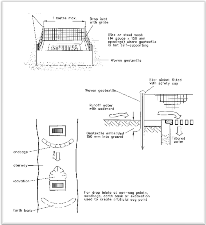
Figure 8 Inlet protection
