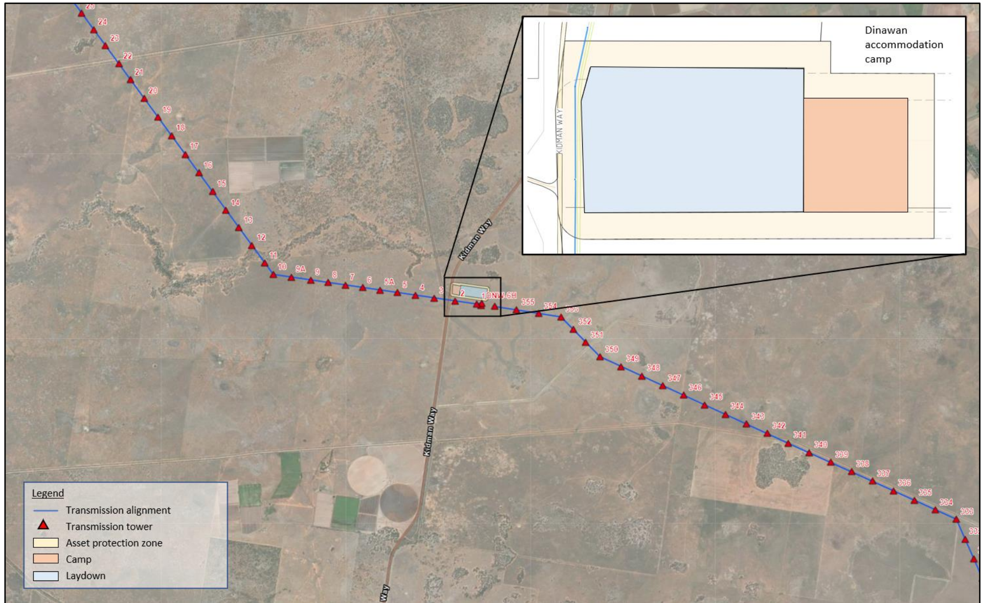
Figure 3.1 - Indicative site boundary of Dinawan accommodation camp
