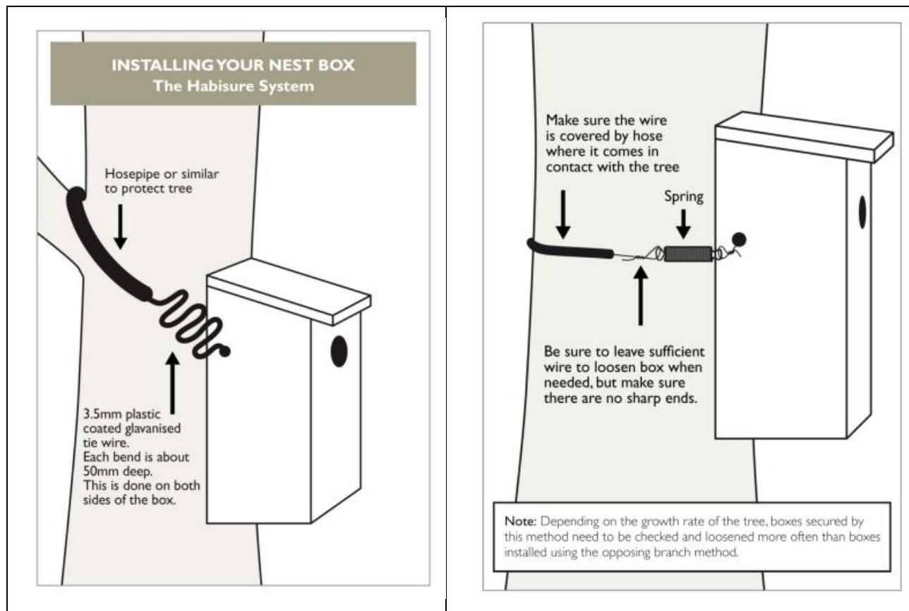
Figure 5.1 - The Habisure © system (from Franks and Franks 2011)
