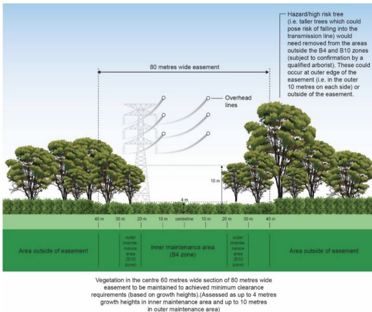
Figure 5.1 - Indicative disturbance area locations and widths applied for 330kV (WSP) (centreline not indicated)
