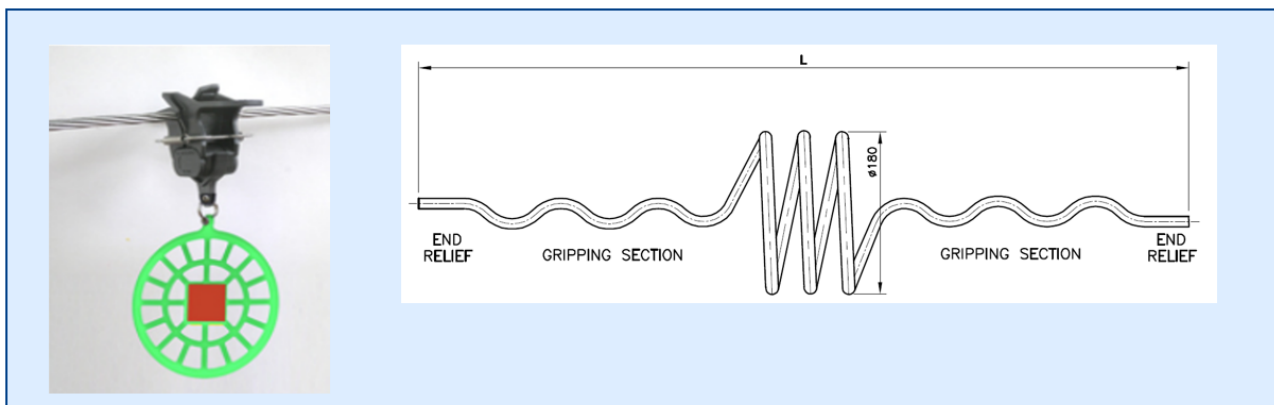
Figure 9.1 - Types of bird diverters
