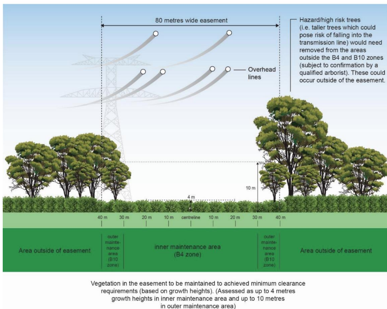
Figure 5.4 - Indicative disturbance area locations and widths applied for a typical 500kV transmission line section (centreline clearing not indicated)
