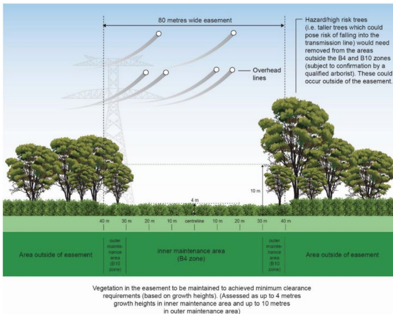
Figure 5.2 - Indicative disturbance area locations and widths applied for 550kV (WSP) (centreline not indicated)
