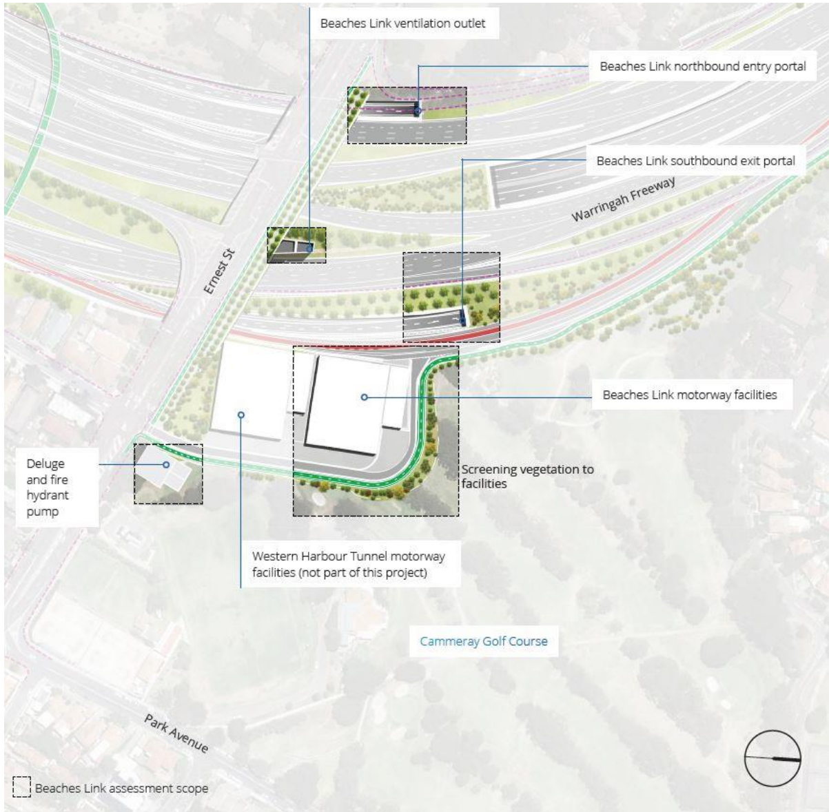
Figure 22-1 North Sydney precinct concept masterplan
