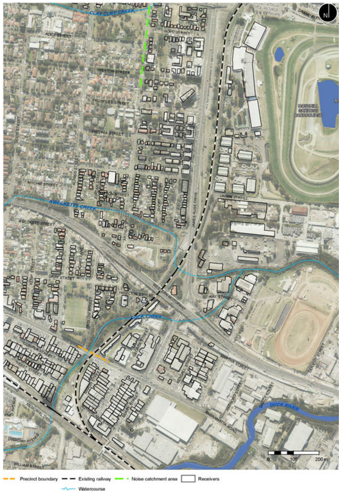
Figure 8: Highly noise affected receivers - Rosehill and Camellia precinct
