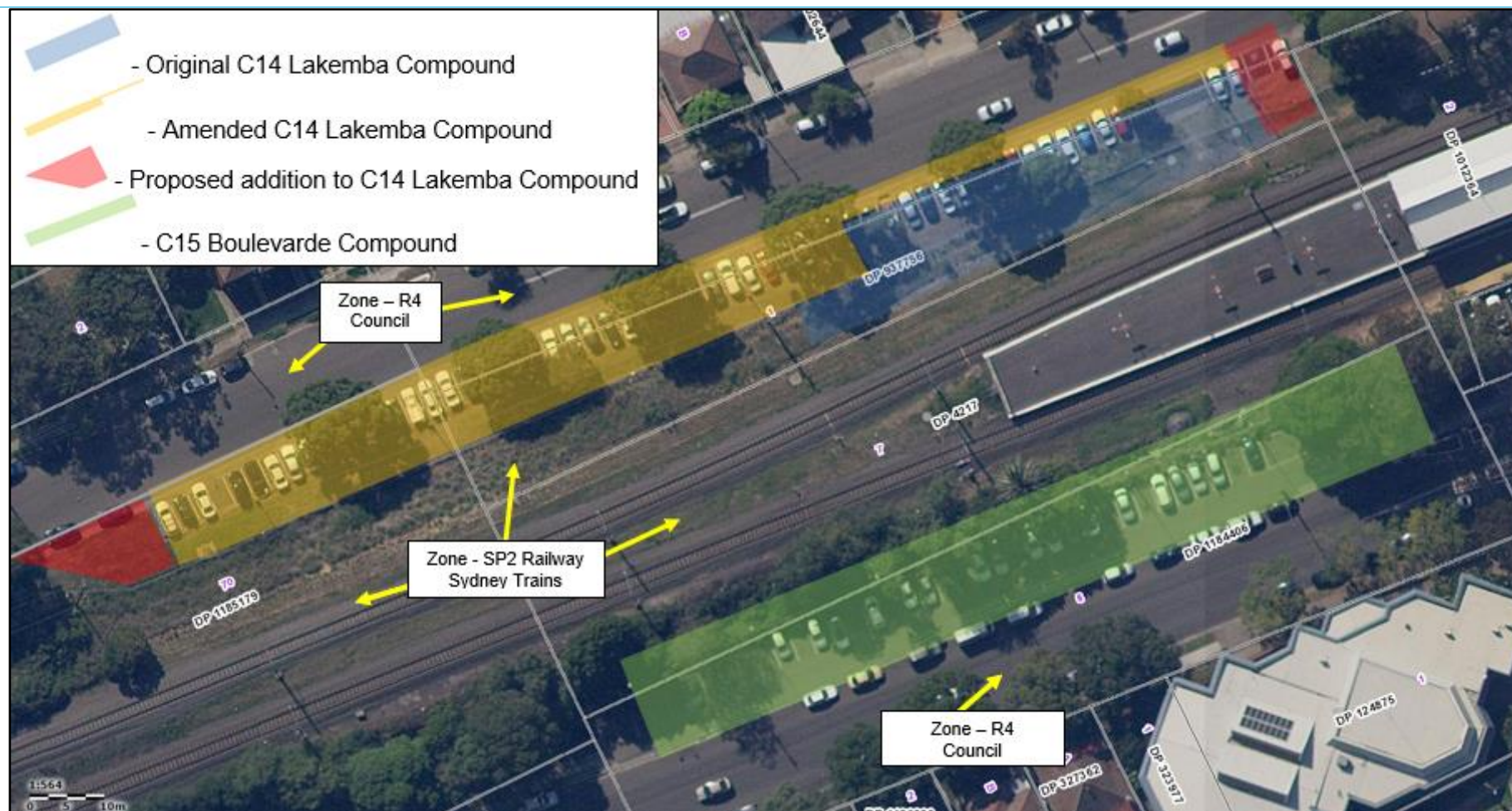
Figure 2 – Worksite boundaries
