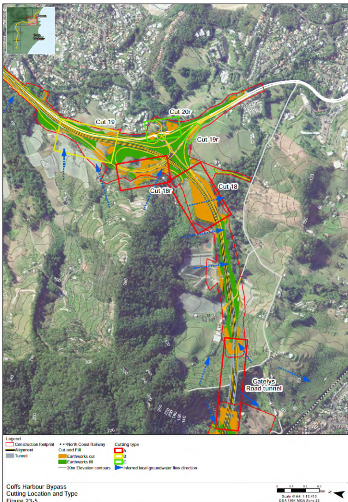
Figure 2-5: Cutting location and type - Coffs Harbour Bypass
