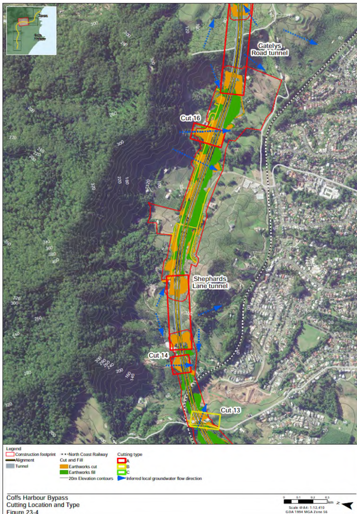
Figure 2-4: Cutting location and type - Coffs Harbour Bypass
