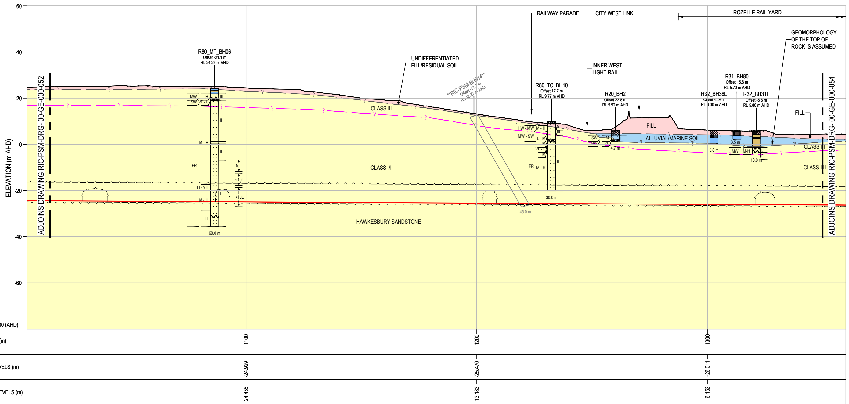
M110 - GEOLOGICAL LONG SECTION SCALE 1:1000
