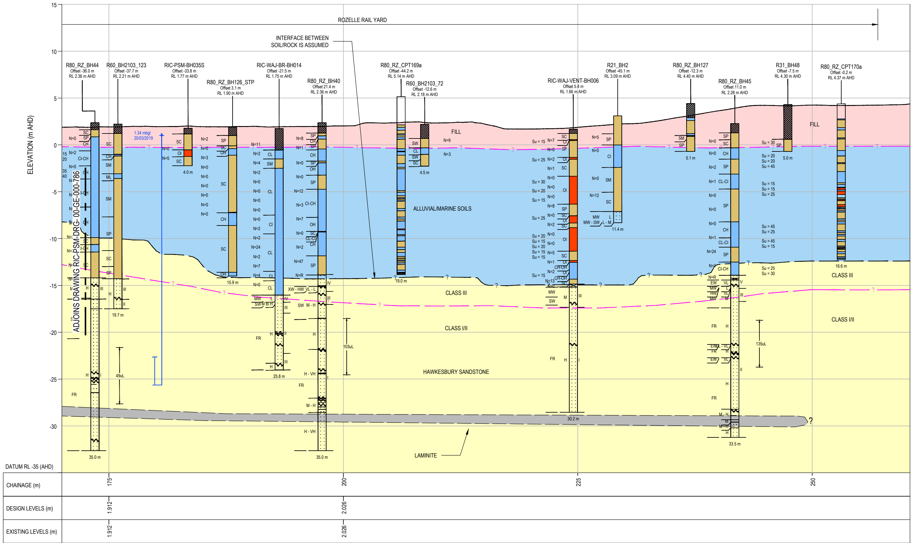
MWCJ WHT TO CWL - GEOLOGICAL LONG SECTION SCALE 1:250
