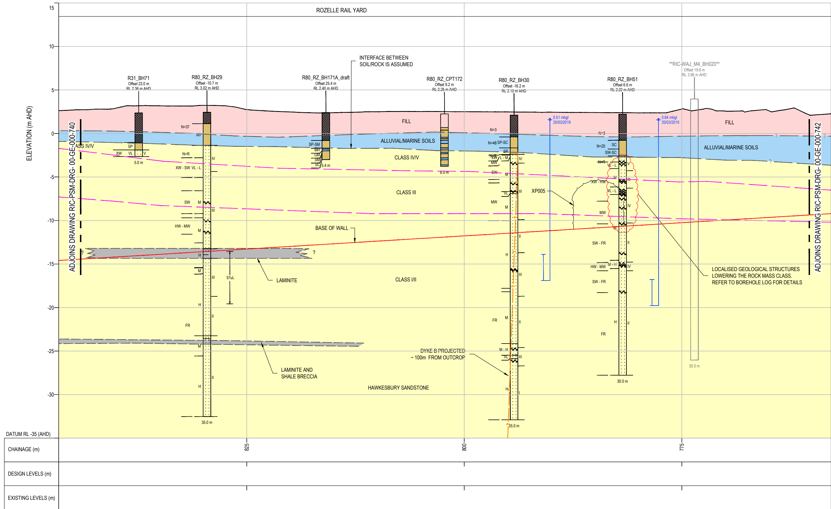
M120 CUT & COVER NORTH WALL - GEOLOGICAL LONG SECTION SCALE 1:250
