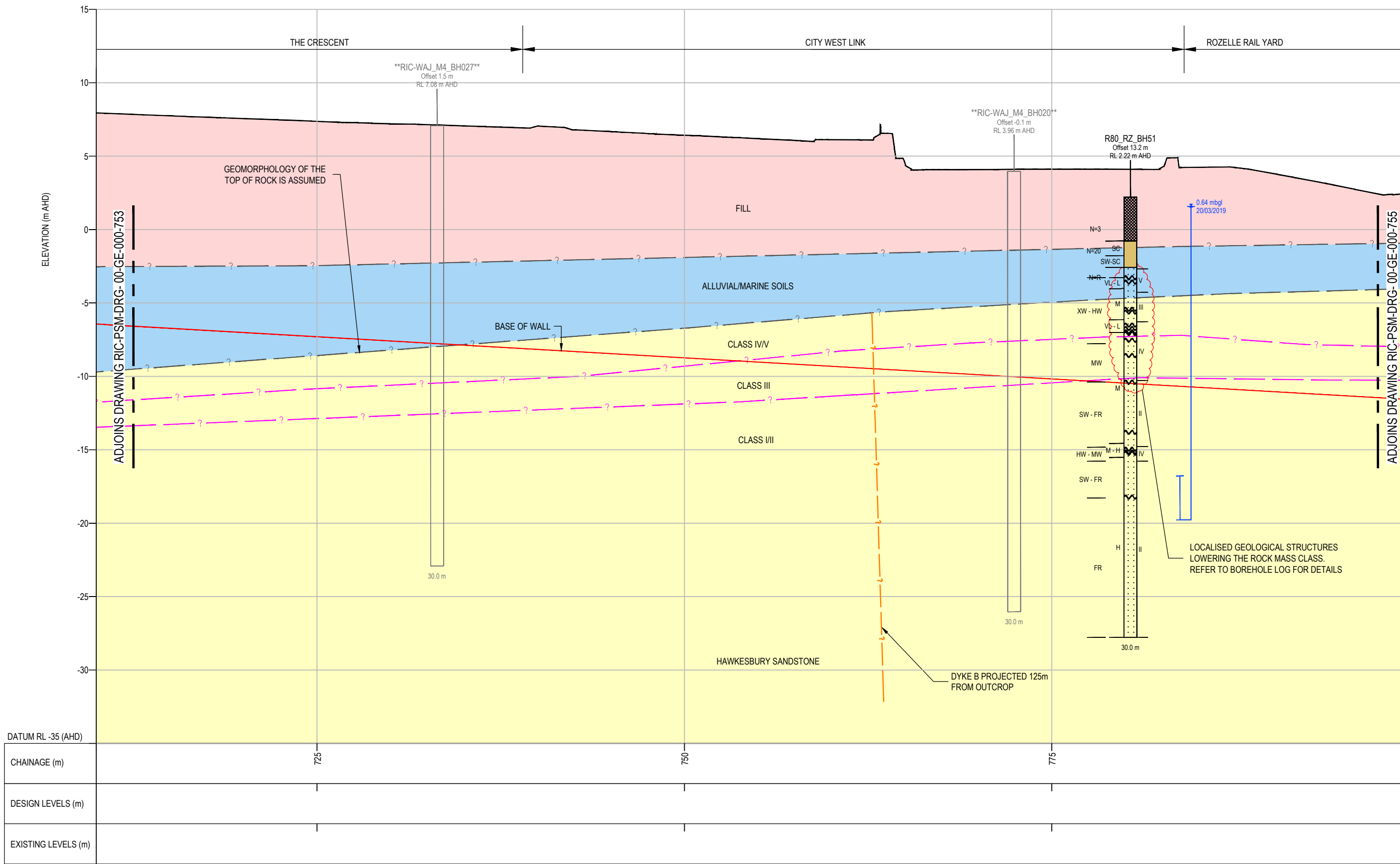
M120 CUT & COVER SOUTH WALL - GEOLOGICAL LONG SECTION SCALE 1:250
