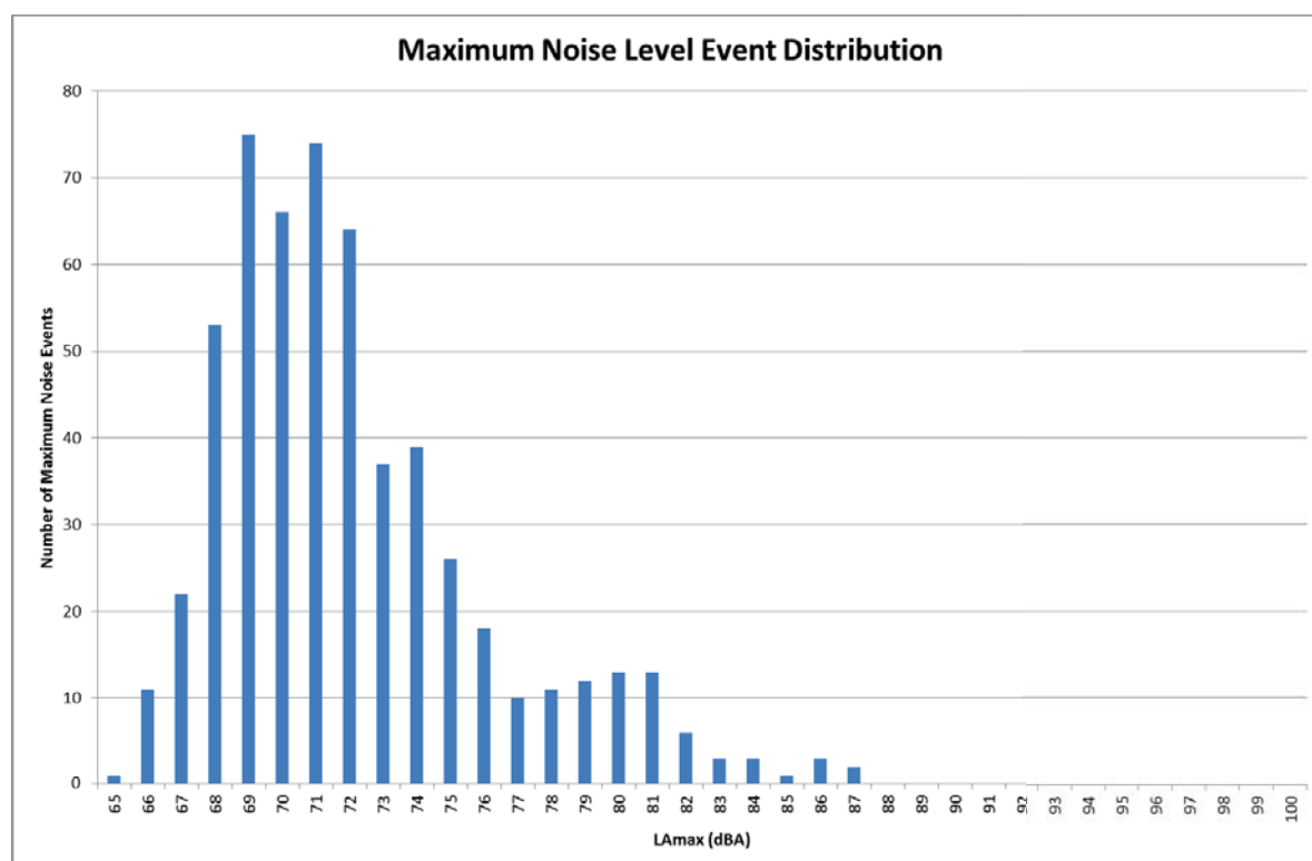
Figure 1 R.01 Maximum Noise Level Event Distribution over Monitoring Period
