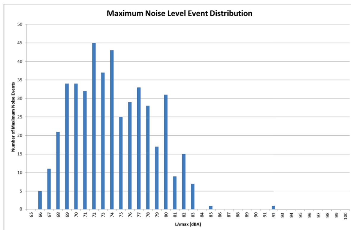
Figure 7 R.07 Maximum Noise Level Event Distribution over Monitoring Period
