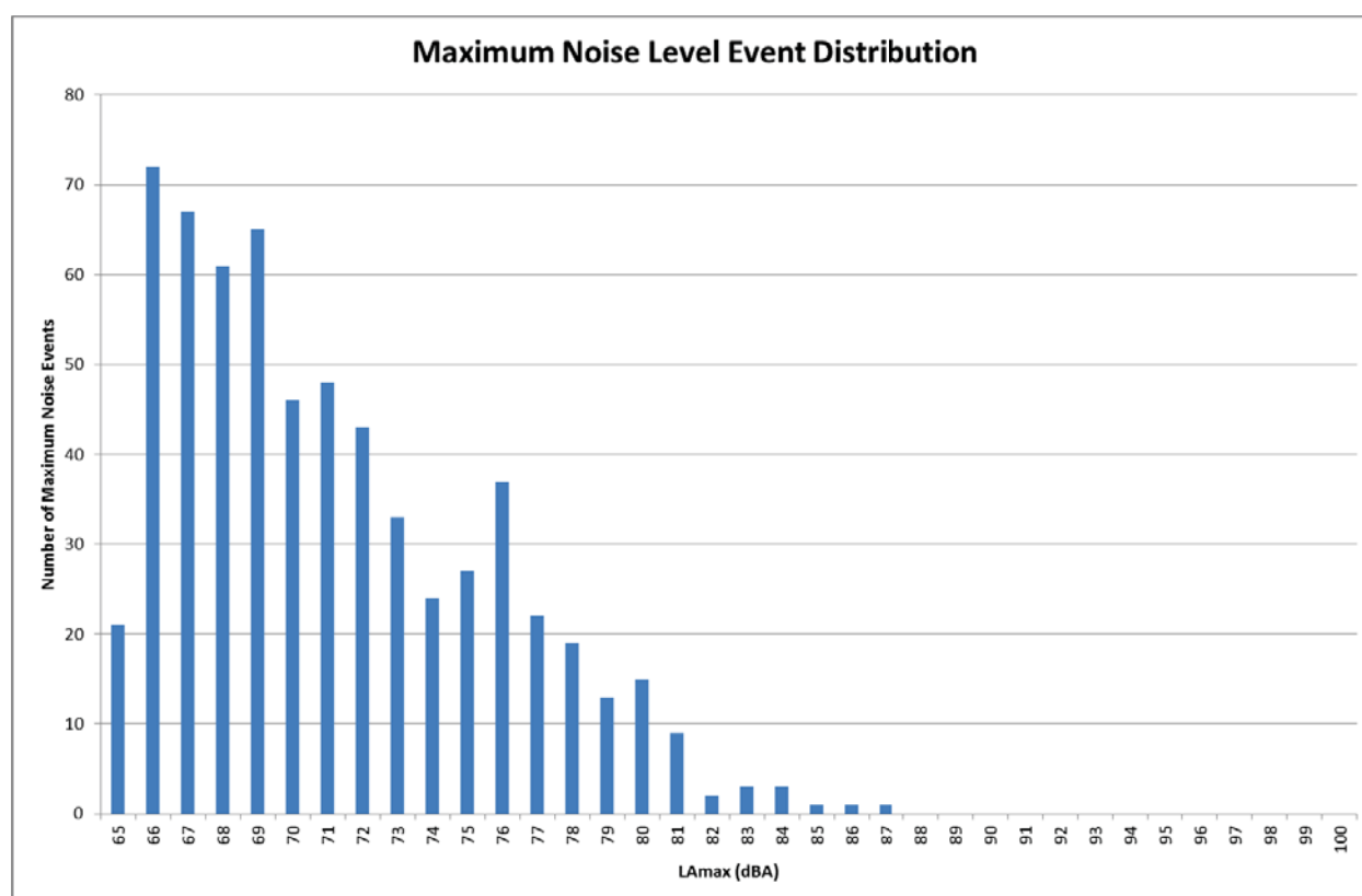
Figure 10 R.10 Maximum Noise Level Event Distribution over Monitoring Period
