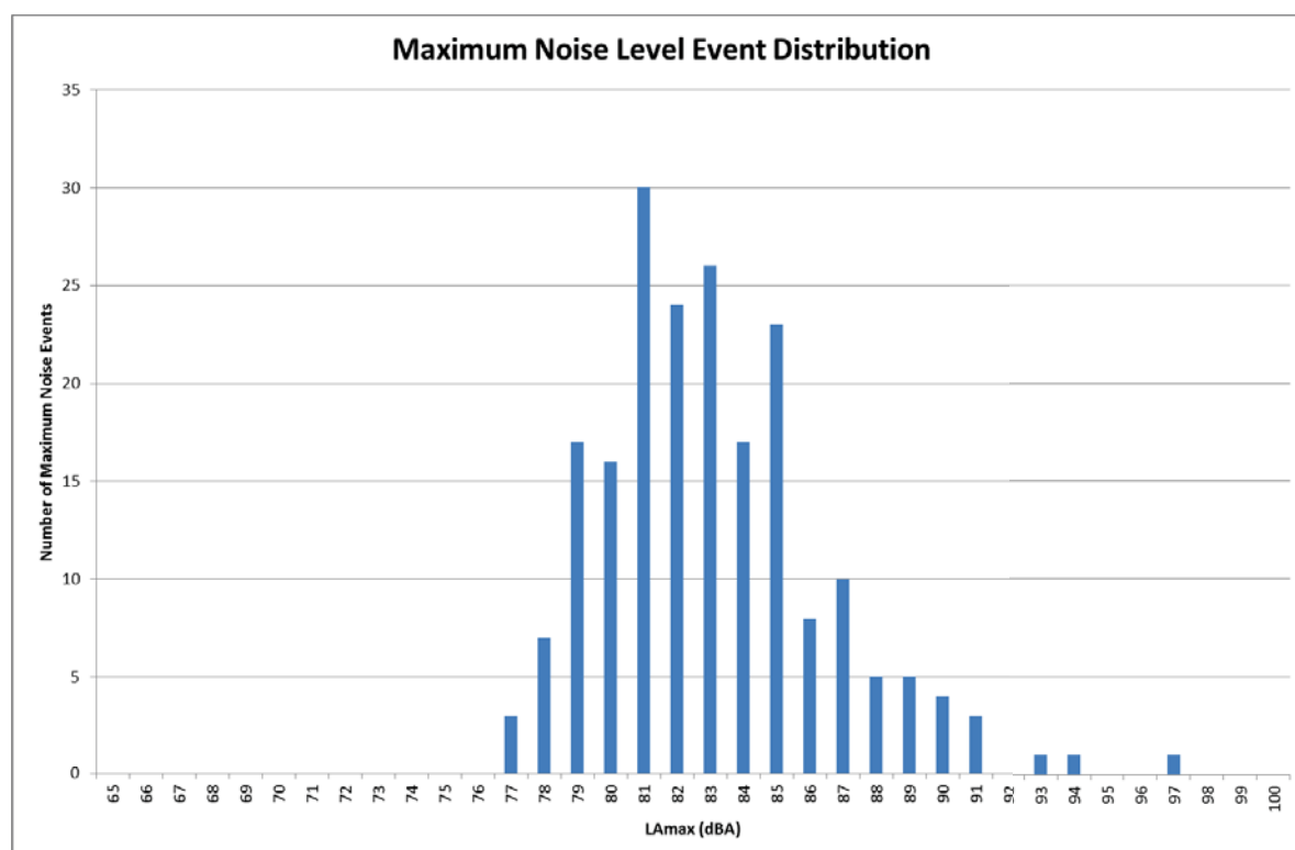
Figure 5 R.05 Maximum Noise Level Event Distribution over Monitoring Period
