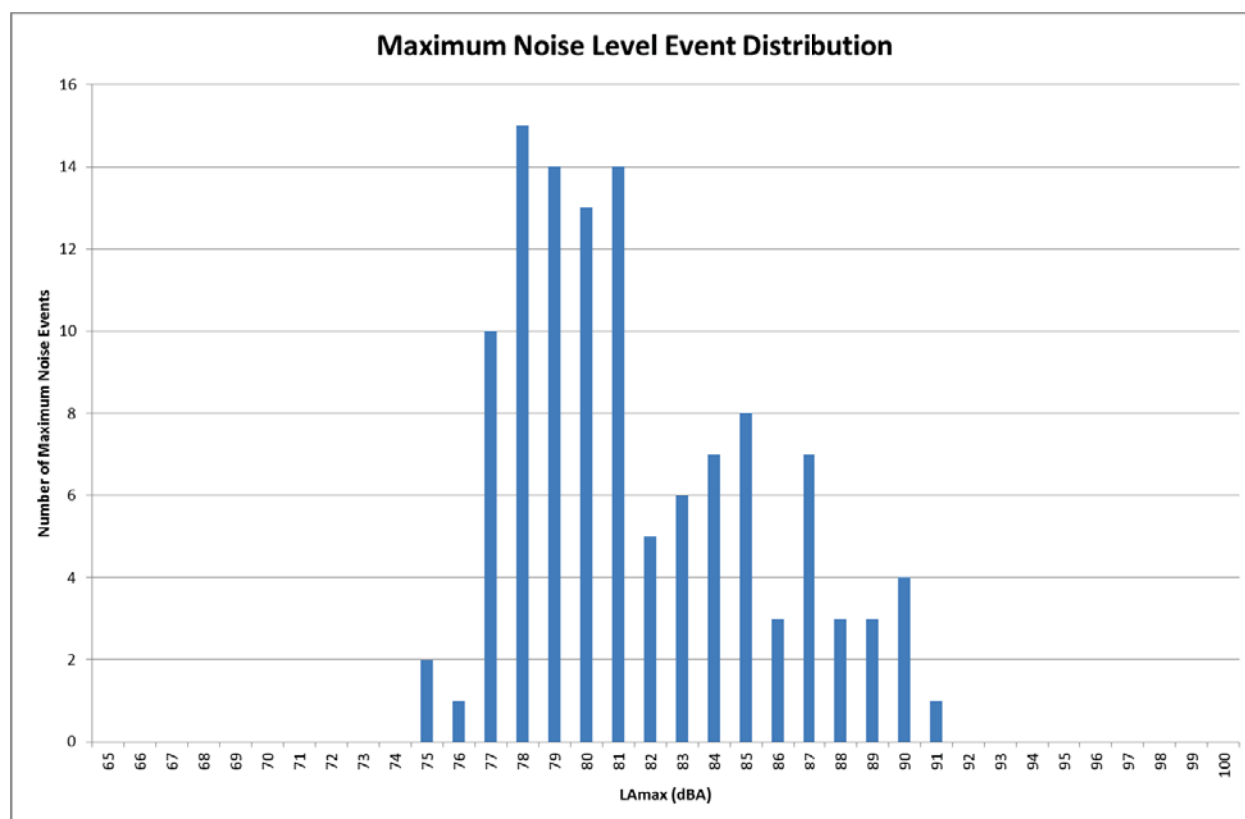
Figure 4 R.04 Maximum Noise Level Event Distribution over Monitoring Period
