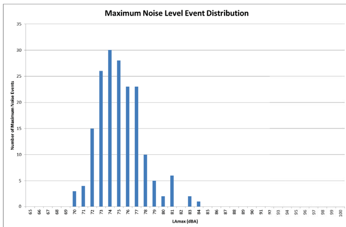
Figure 6 R.06 Maximum Noise Level Event Distribution over Monitoring Period
