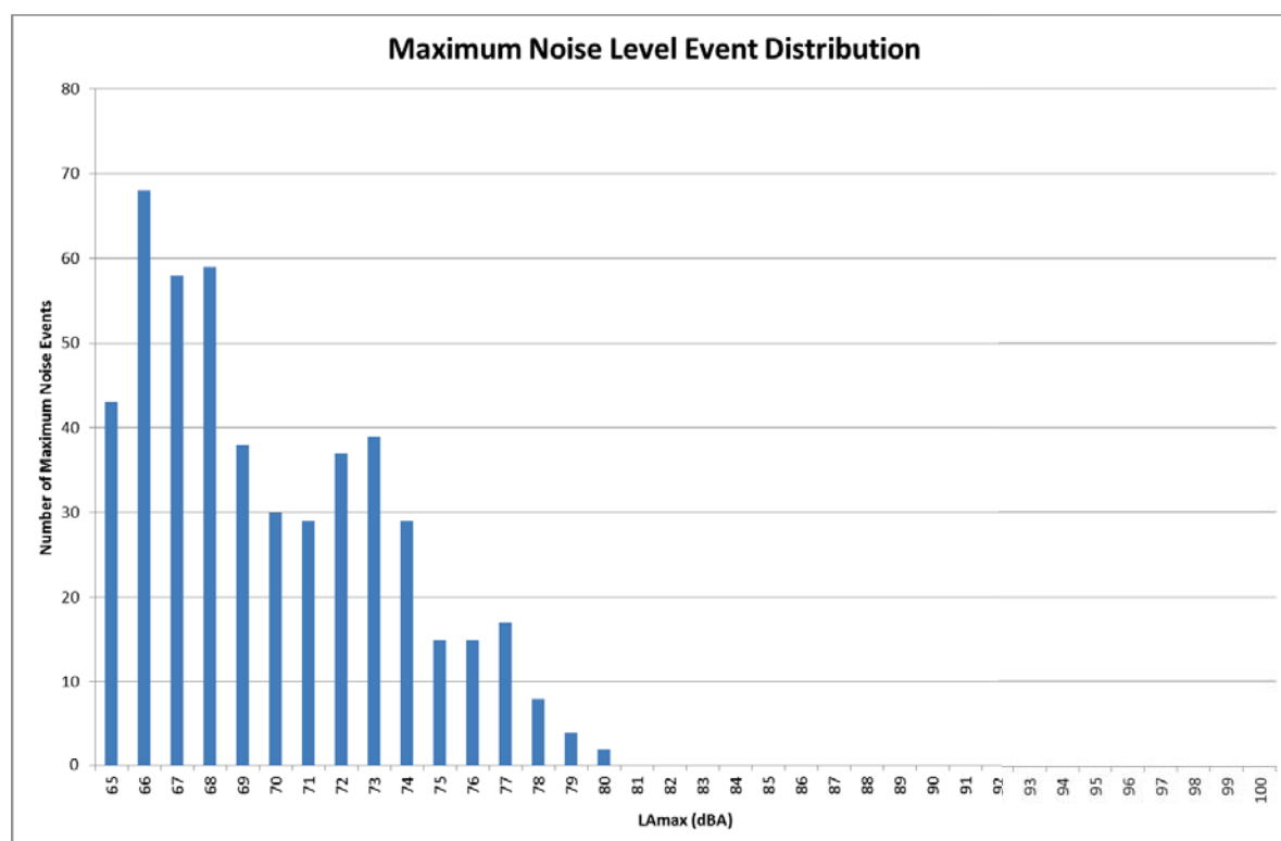
Figure 9 R.09 Maximum Noise Level Event Distribution over Monitoring Period
