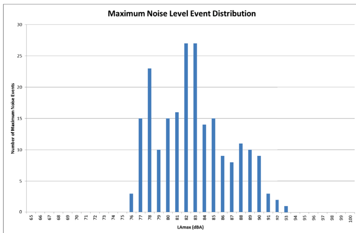
Figure 3 R.03 Maximum Noise Level Event Distribution over Monitoring Period
