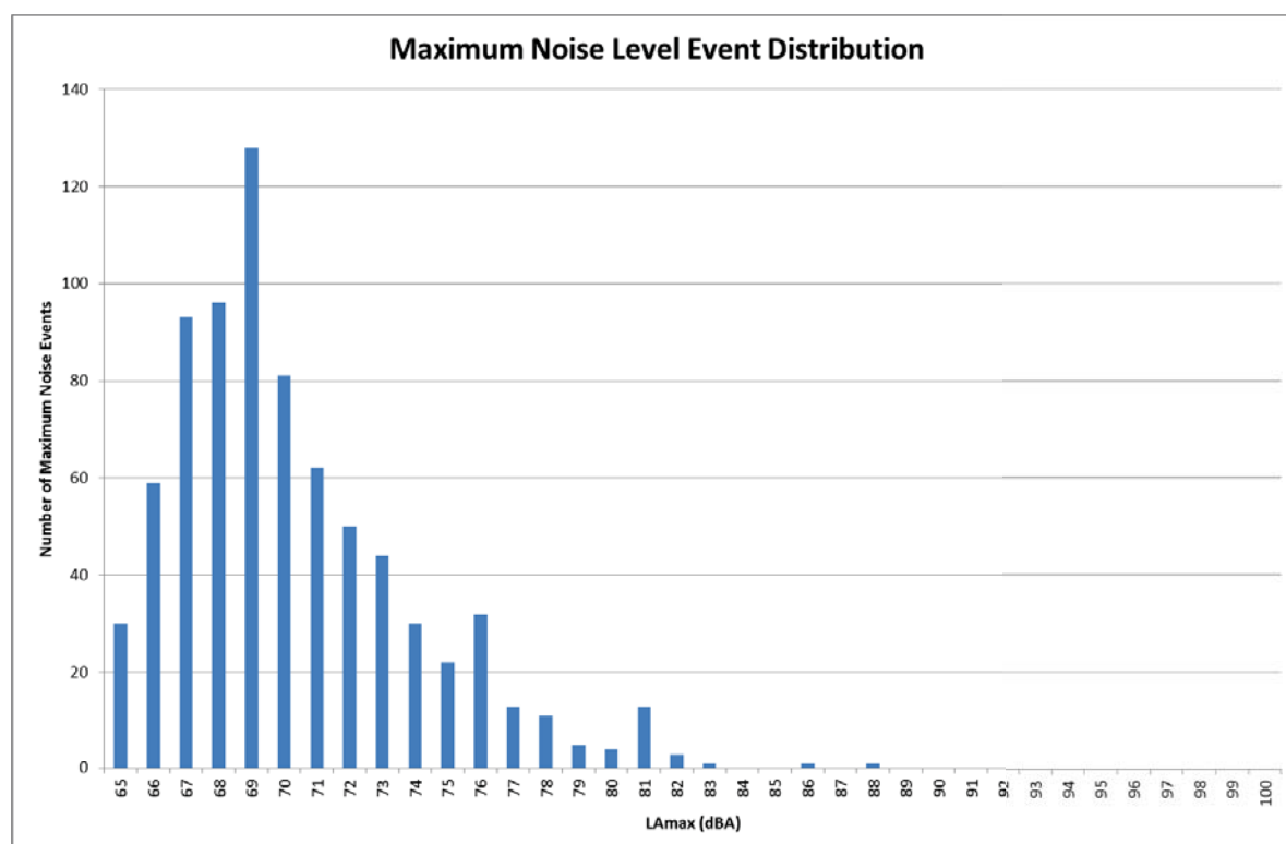
Figure 8 R.08 Maximum Noise Level Event Distribution over Monitoring Period
