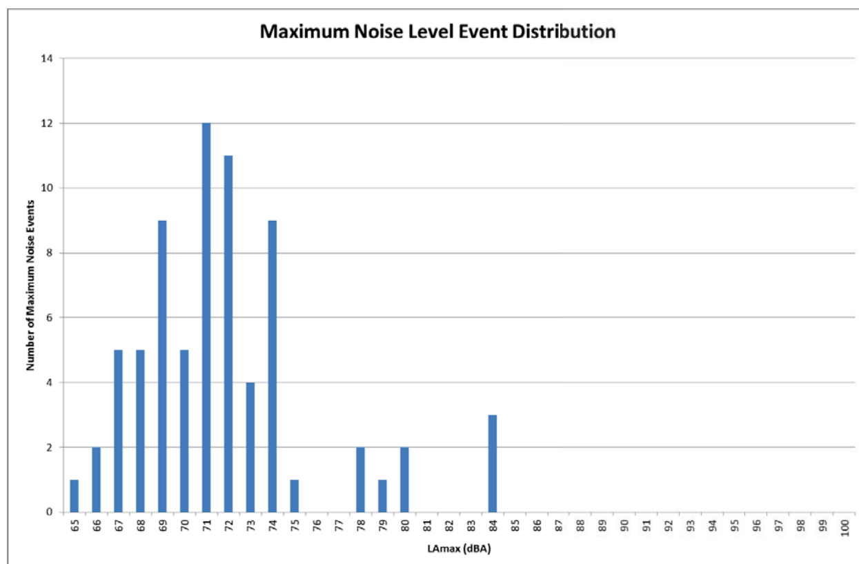
Figure 2 R.02 Maximum Noise Level Event Distribution over Monitoring Period
