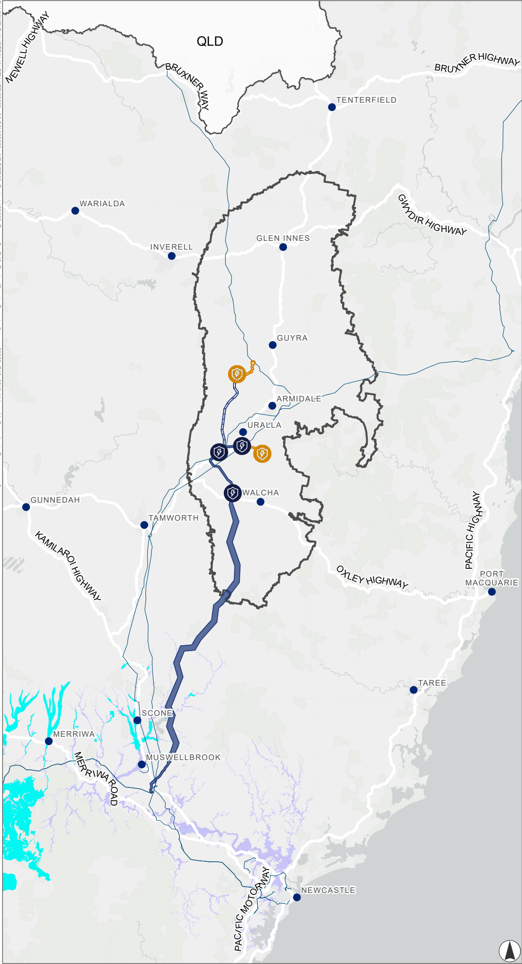
FIGURE 6-12 Vulnerable Groundwater Resources and Groundwater Sharing Plans
