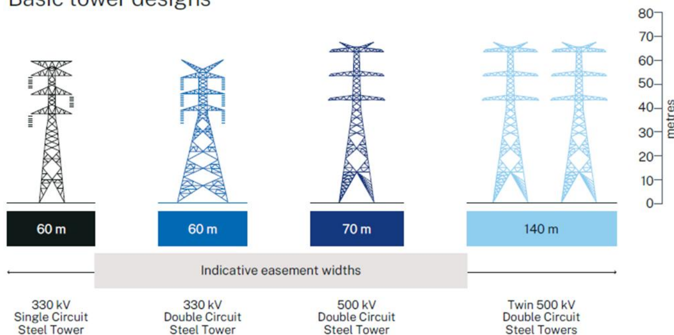
Figure 3-2: Indicative concept design and easement widths for the transmission line towers
