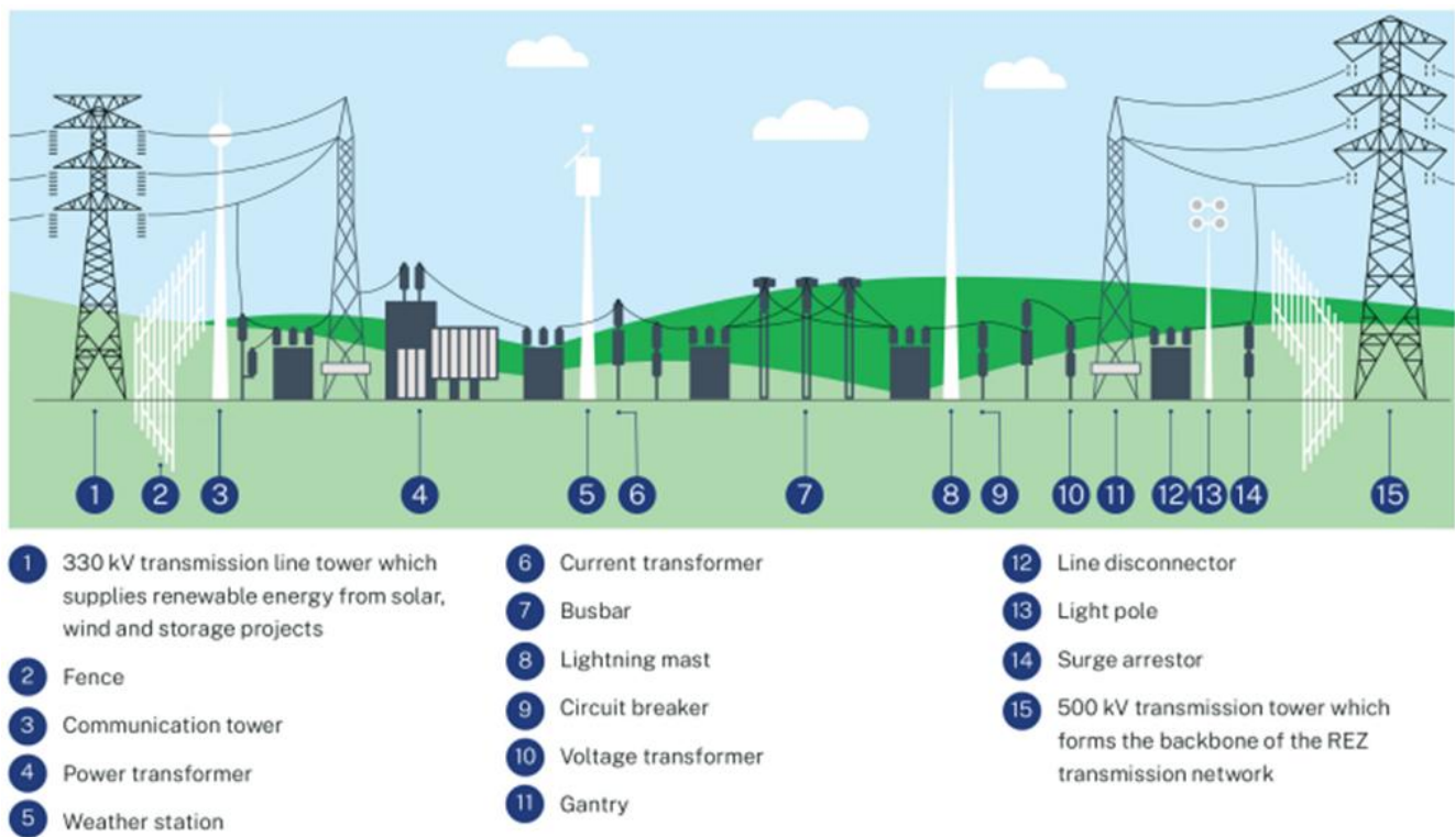
Figure 3-3: Indicative energy hub arrangement
