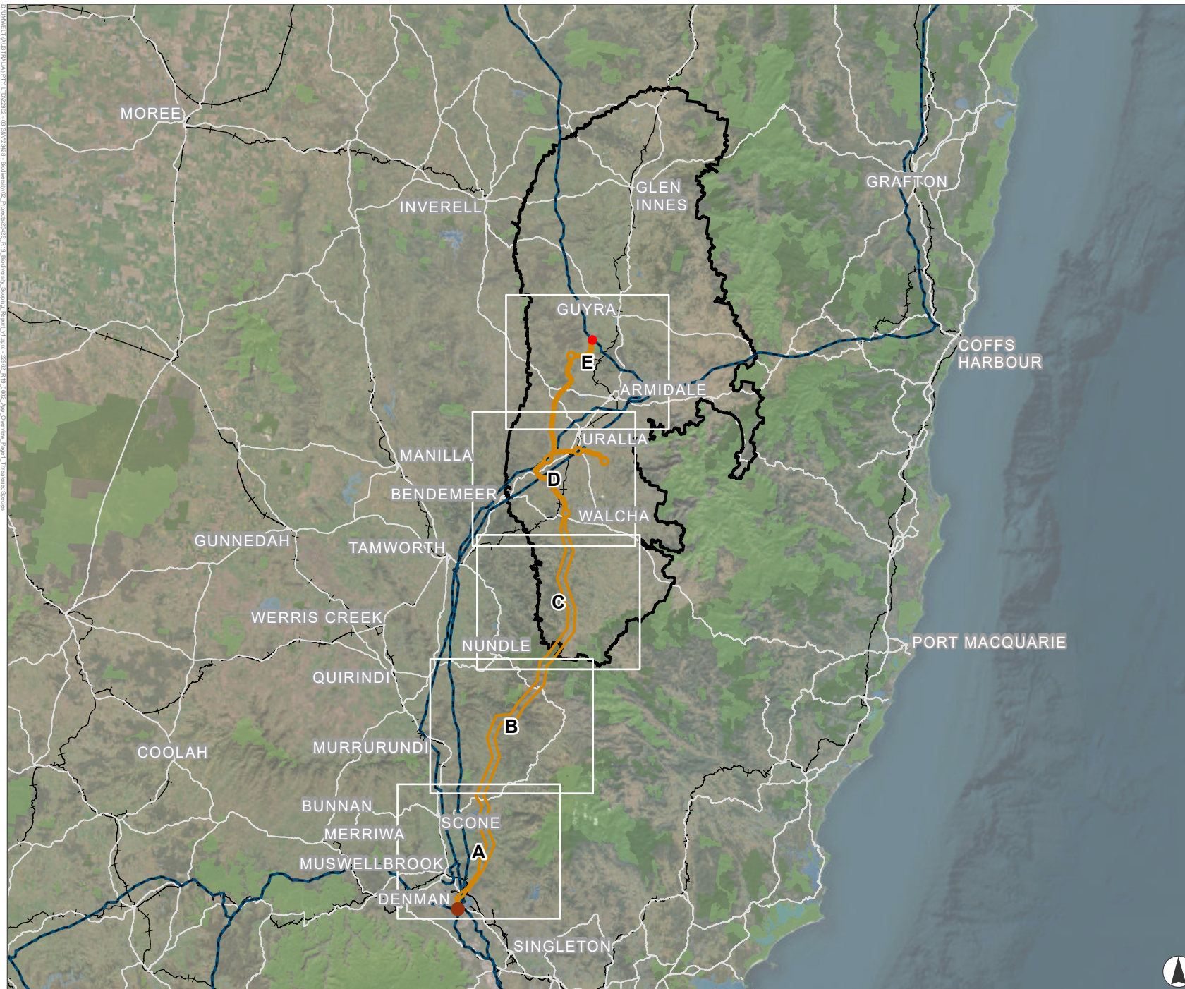
FIGURE 6-2 Threatened Species Records
