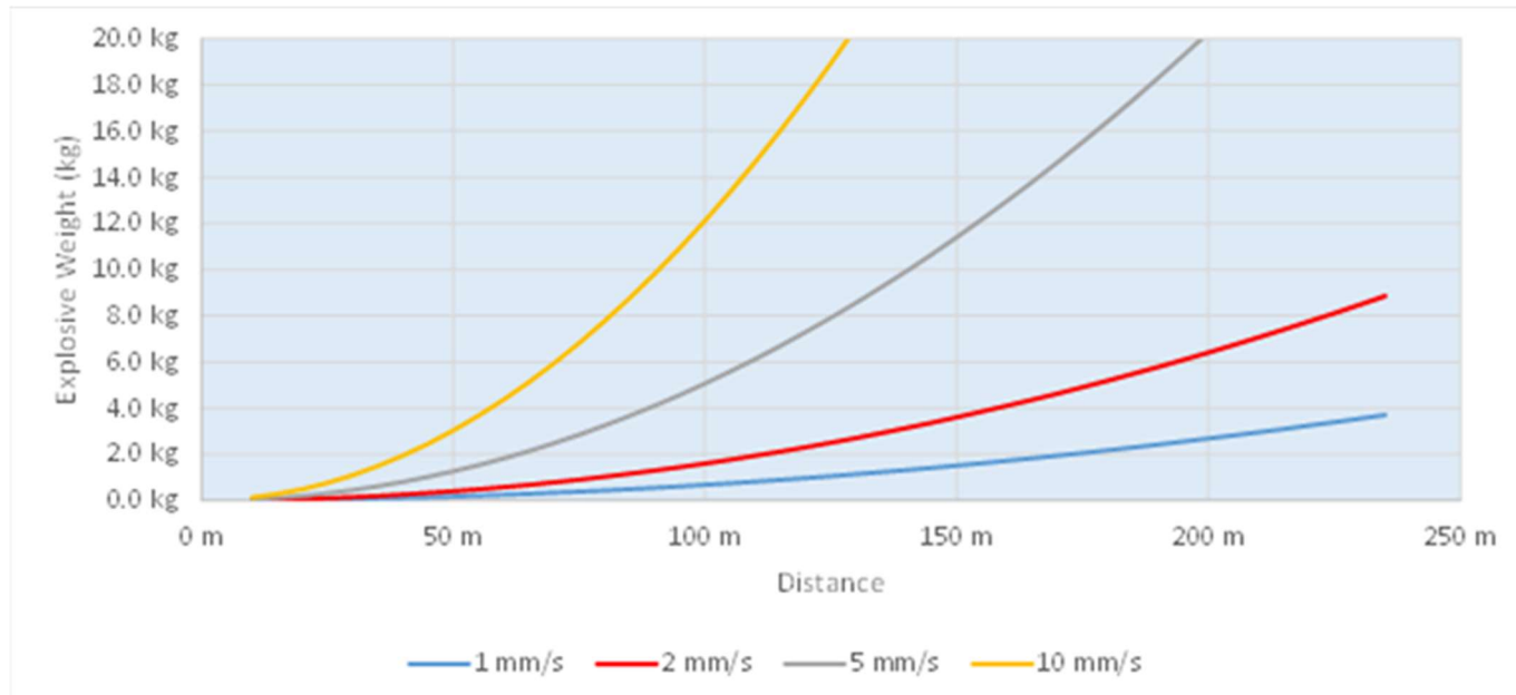
Figure 4: Vibration level as a function of distance from varying explosive quantities per delay for compliance with 10mm/s
