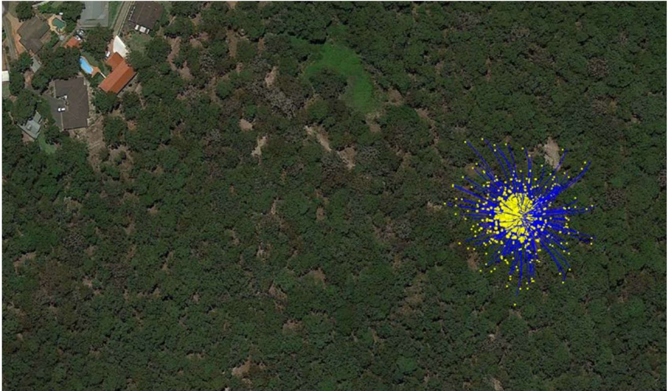
Figure 4: Predicted flyrock locations from blasting with a 89mm diameter blast-hole and 7.5 metre bench. The predicted locations are shown as the yellow markers.
