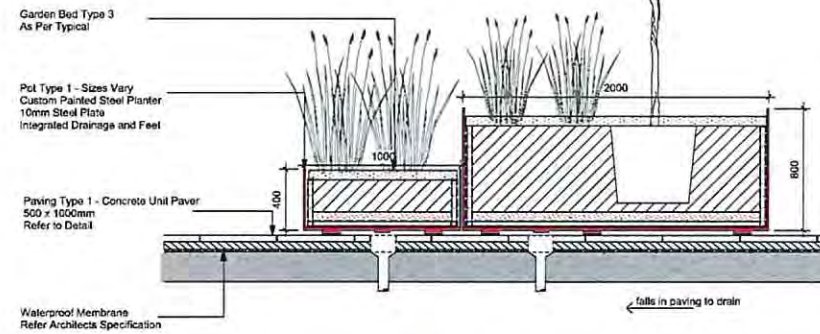
6 GB3- Independent Steel Planter - Entry Courtyards 1:20
