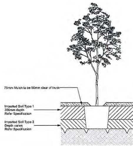
1 Typical Tree Planting 1:20
