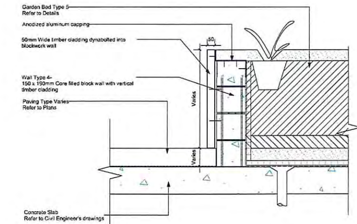
5 Wall Type 4 - Blockwork Wall with Timber Cladding 1:10
