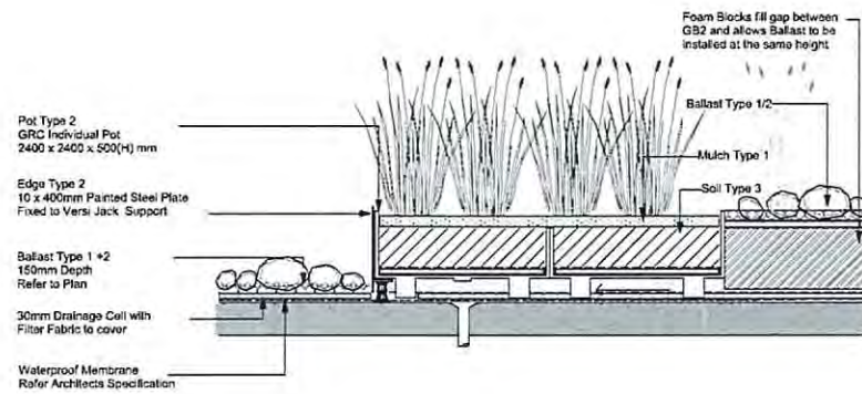
5 GB2 - Independent Planter over Slab - Internal Only 1:20
