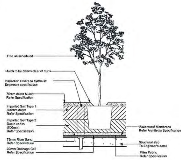
2 Advanced Tree on Slab 1:20
