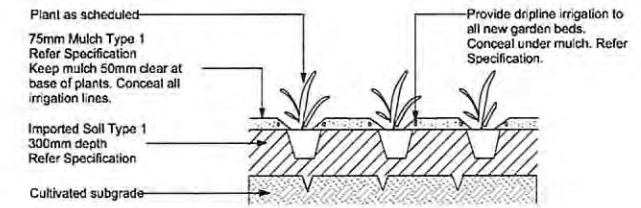
4 GB1- Garden Bed on Grade 1:20
