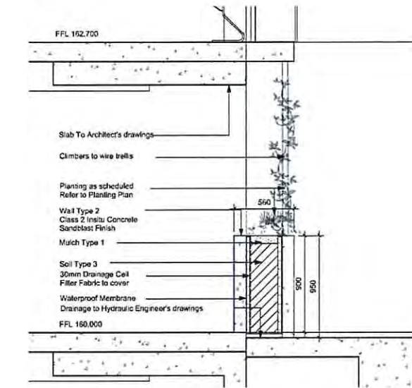
4 GB1- Garden Bed on Grade 1:20
