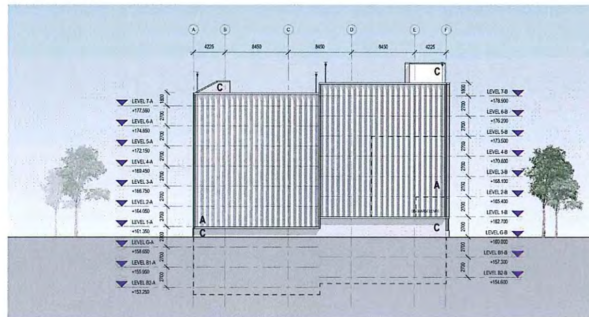
SOUTH ELEVATION
