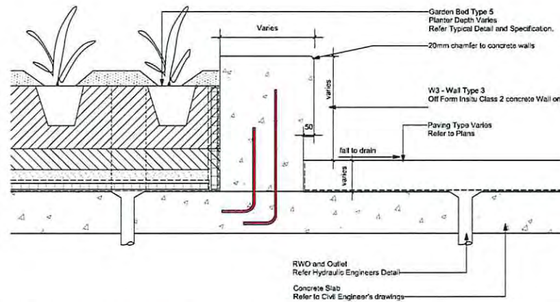
4 Wall Type 3 - Class 2 Insitu Concrete Wall on Slab 1:10
