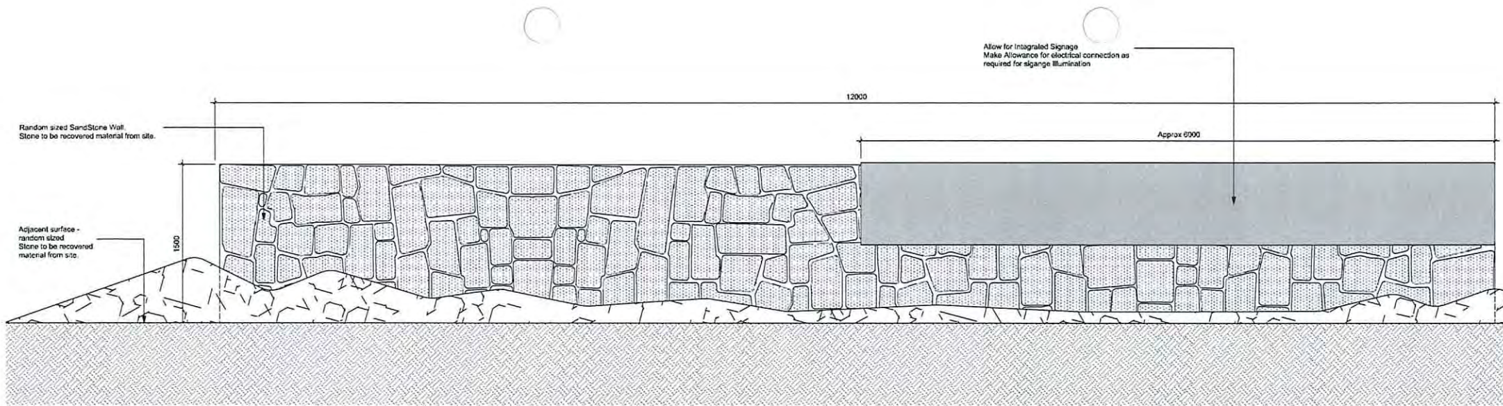
1 Wall Type 1 - Stone Entrance Wall (Indicative Only) 1:20
