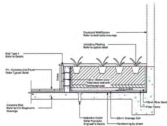
8 GB5 - Garden Bed on Slab - Mental Health Building 1:20
