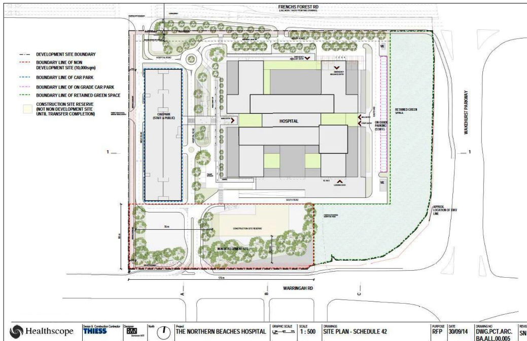
Figure 1 Masterplan (Thiess)
