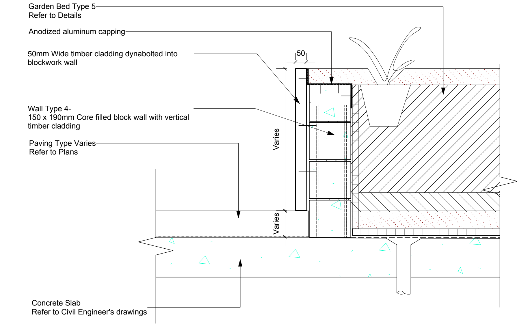
5 Wall Type 4 - Blockwork Wall with Timber Cladding 1:10
