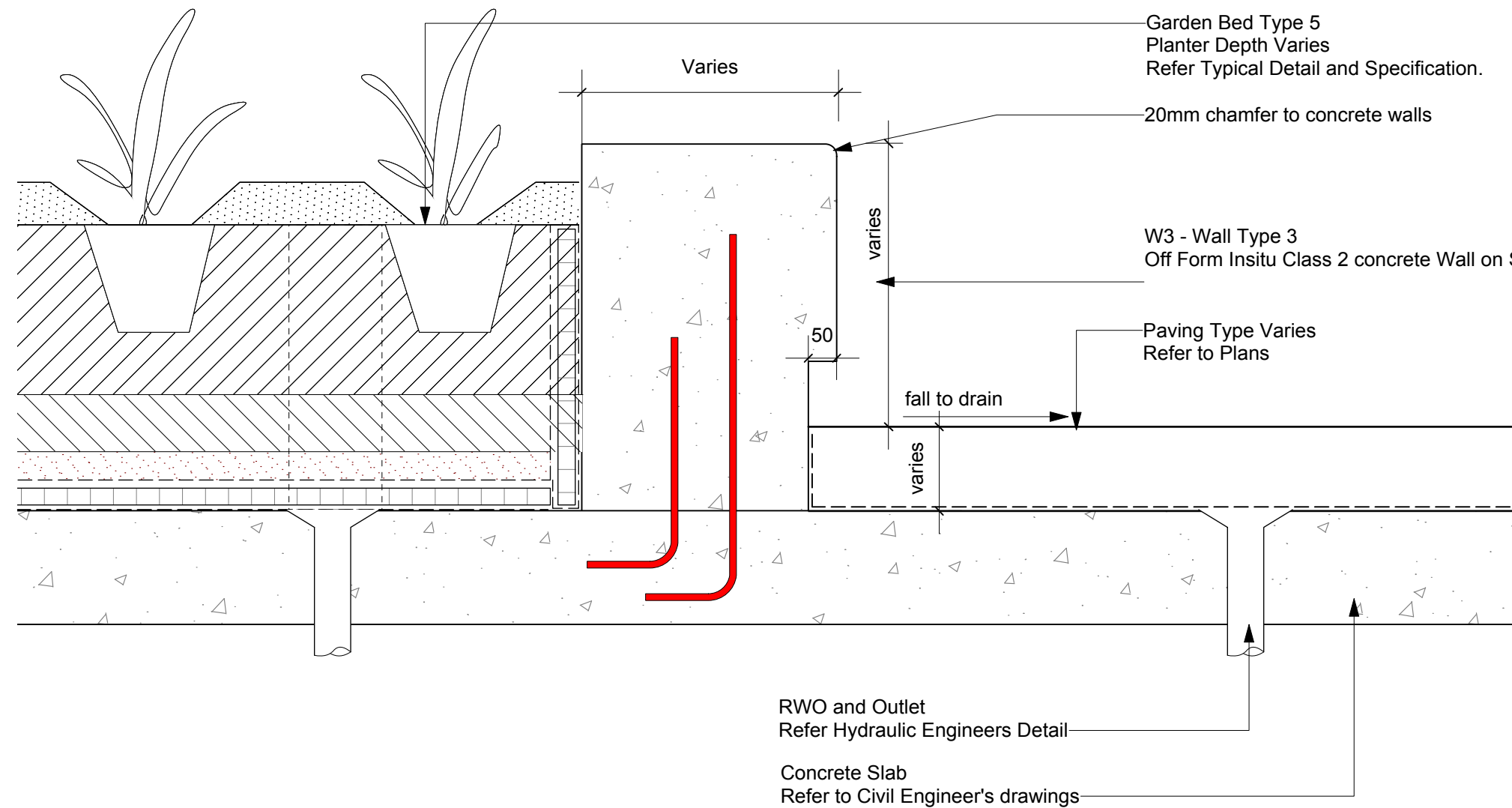
4 Wall Type 3 - Class 2 Insitu Concrete Wall on Slab 1:10
