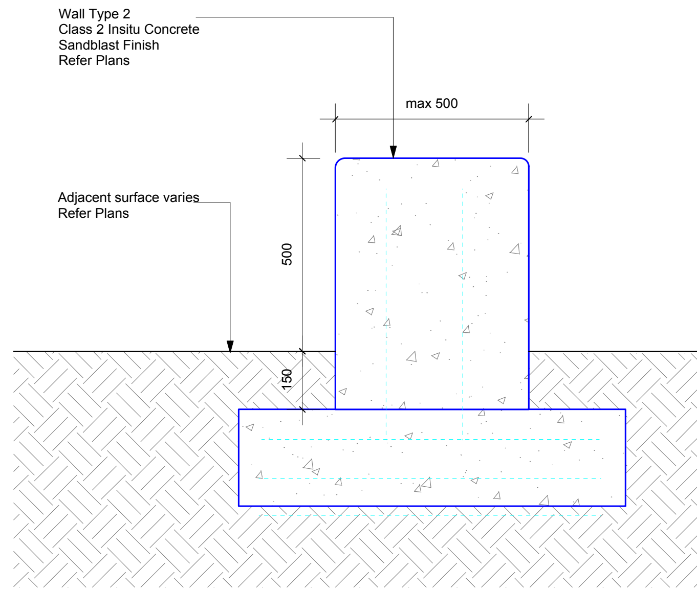
3 Wall Type 2 - Class 2 Insitu Concrete Wall on Grade 1:10
