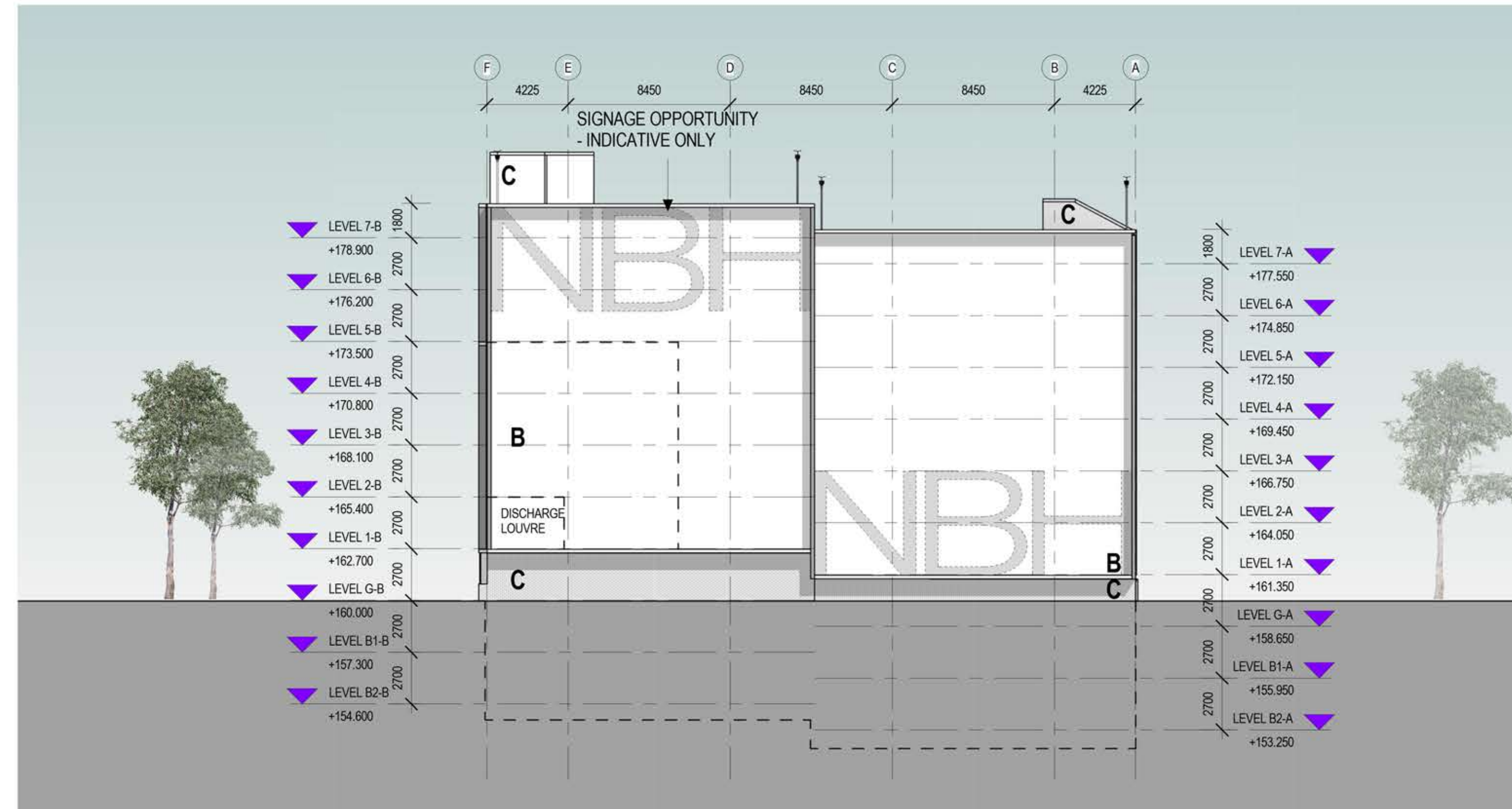
NORTH ELEVATION
