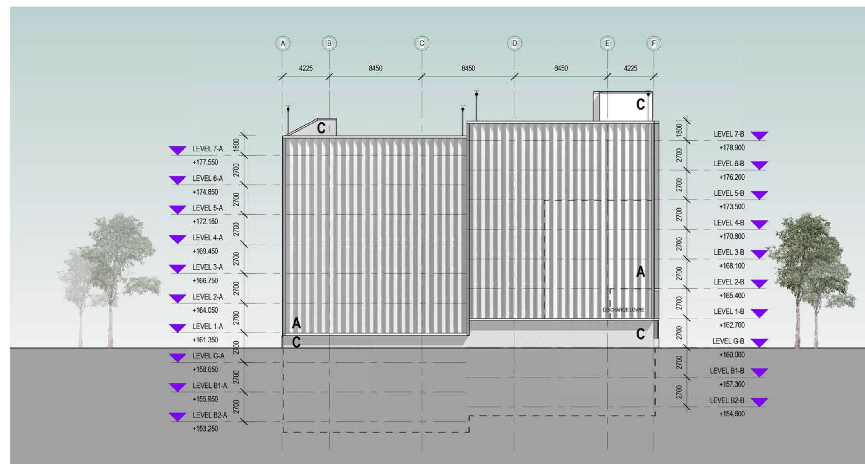
SOUTH ELEVATION
