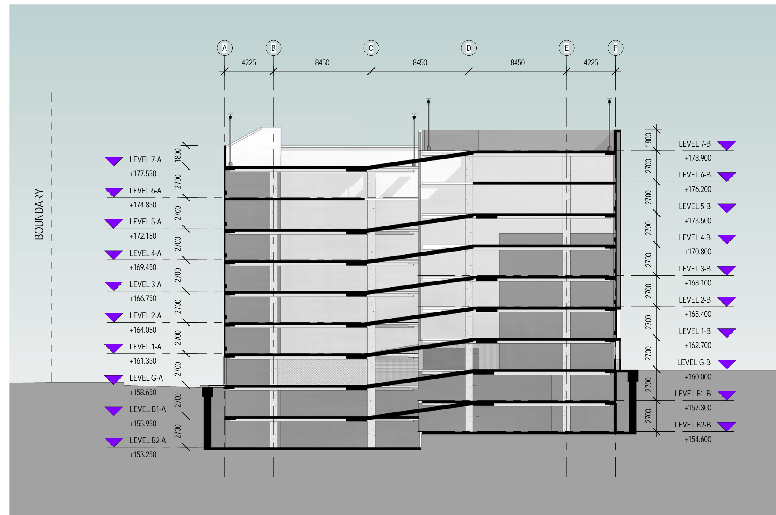
SECTION
