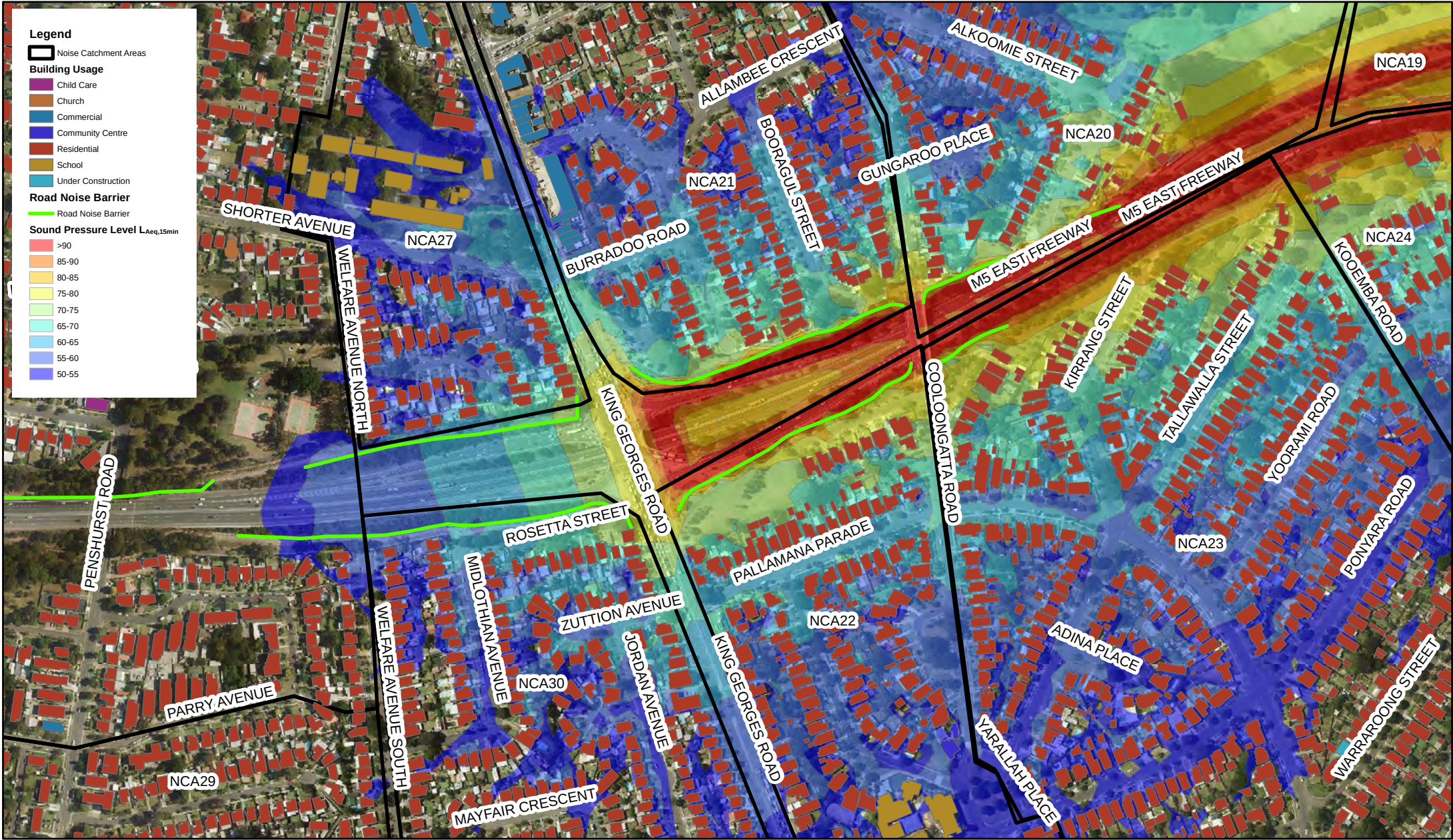
WestConnex Stage 2 - Construction Noise Assessment Surface works - M5 East Motorway road widening and realignment (Rock hammering only) - Earthworks - Day
