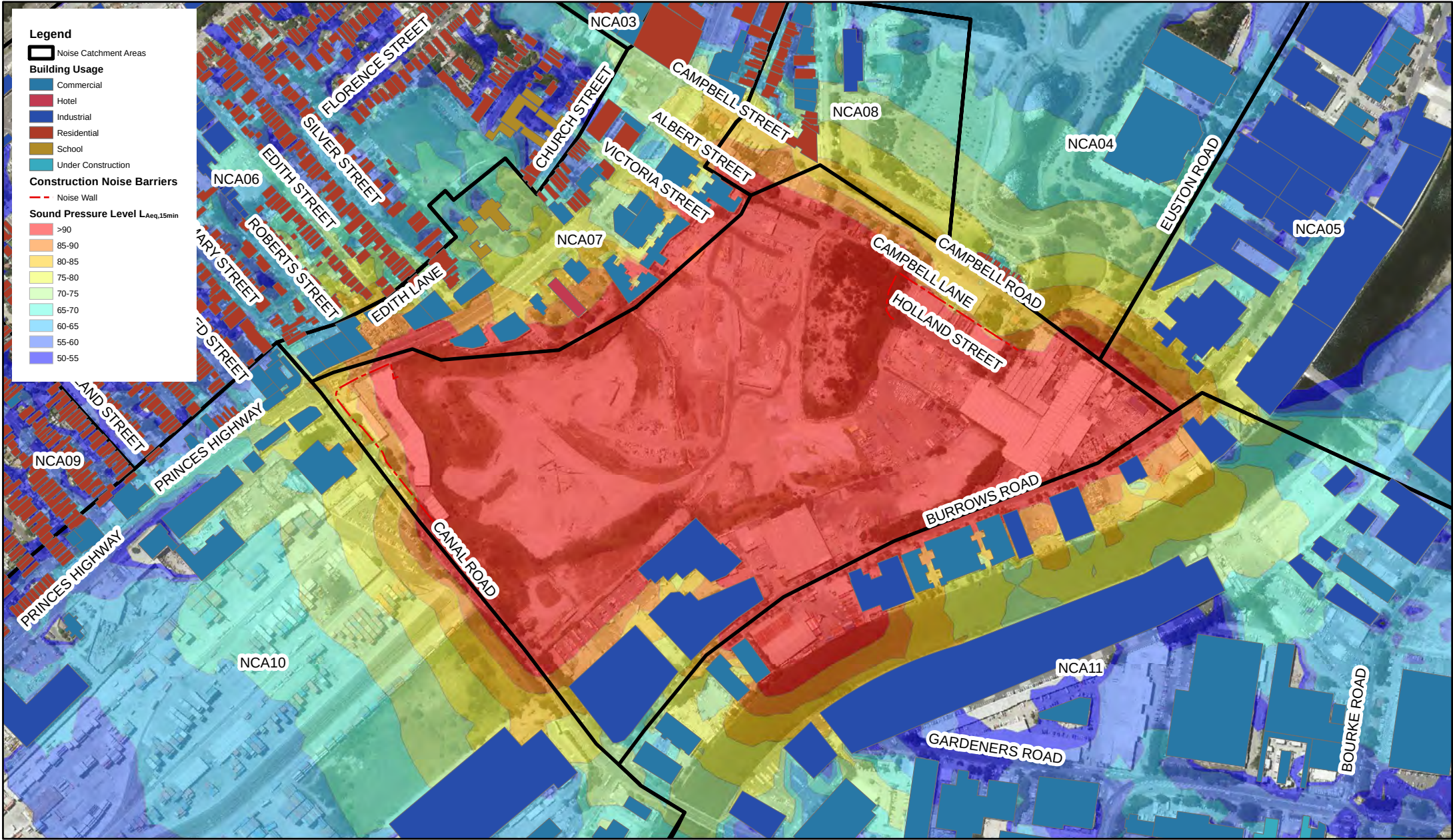
WestConnex Stage 2 - Construction Noise Assessment Surface works - Construction of SPI - Earthworks (Rock hammering only) - Day
