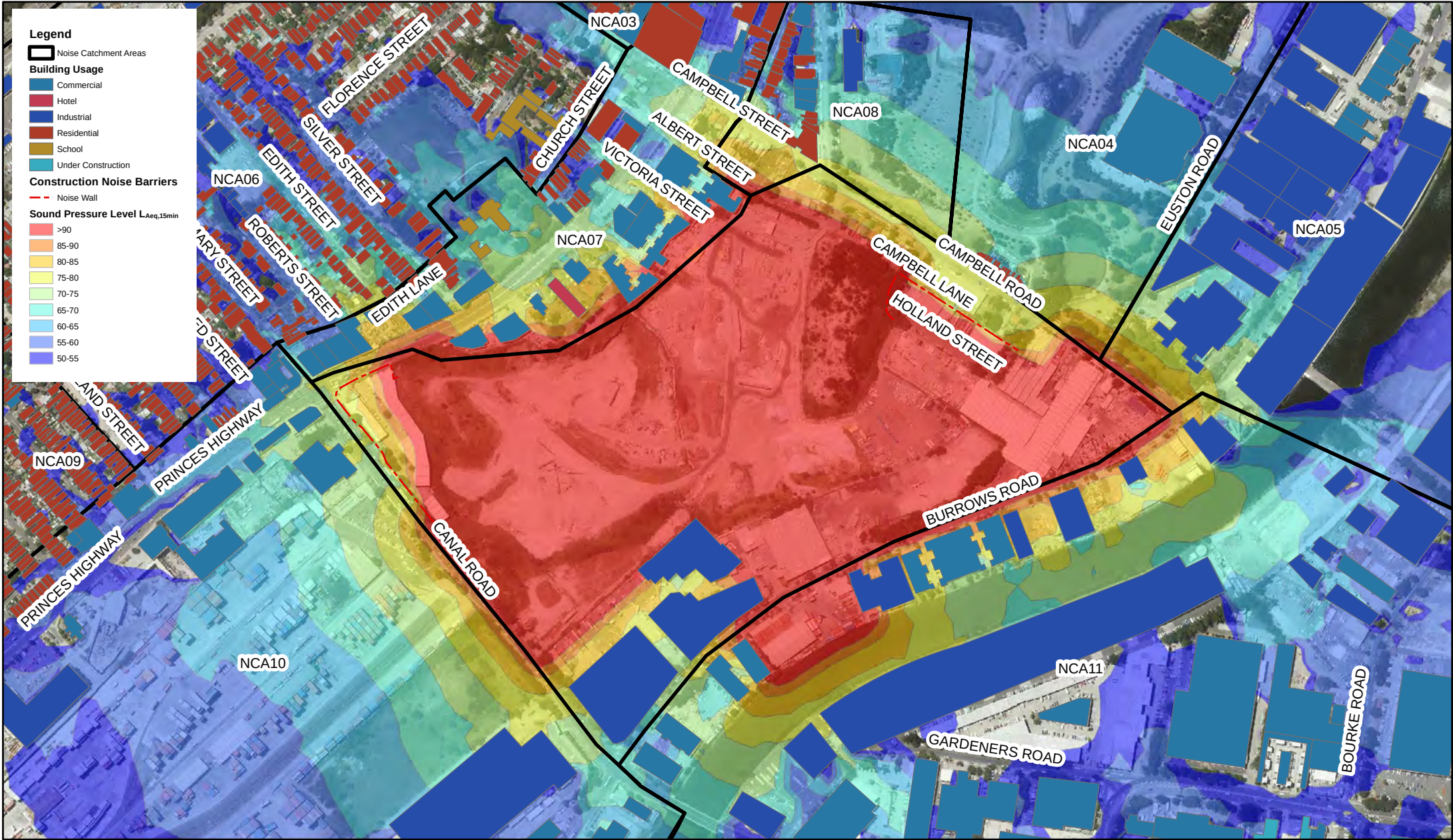
WestConnex Stage 2 - Construction Noise Assessment Surface works - Construction of SPI - Road tie-in works - Day
