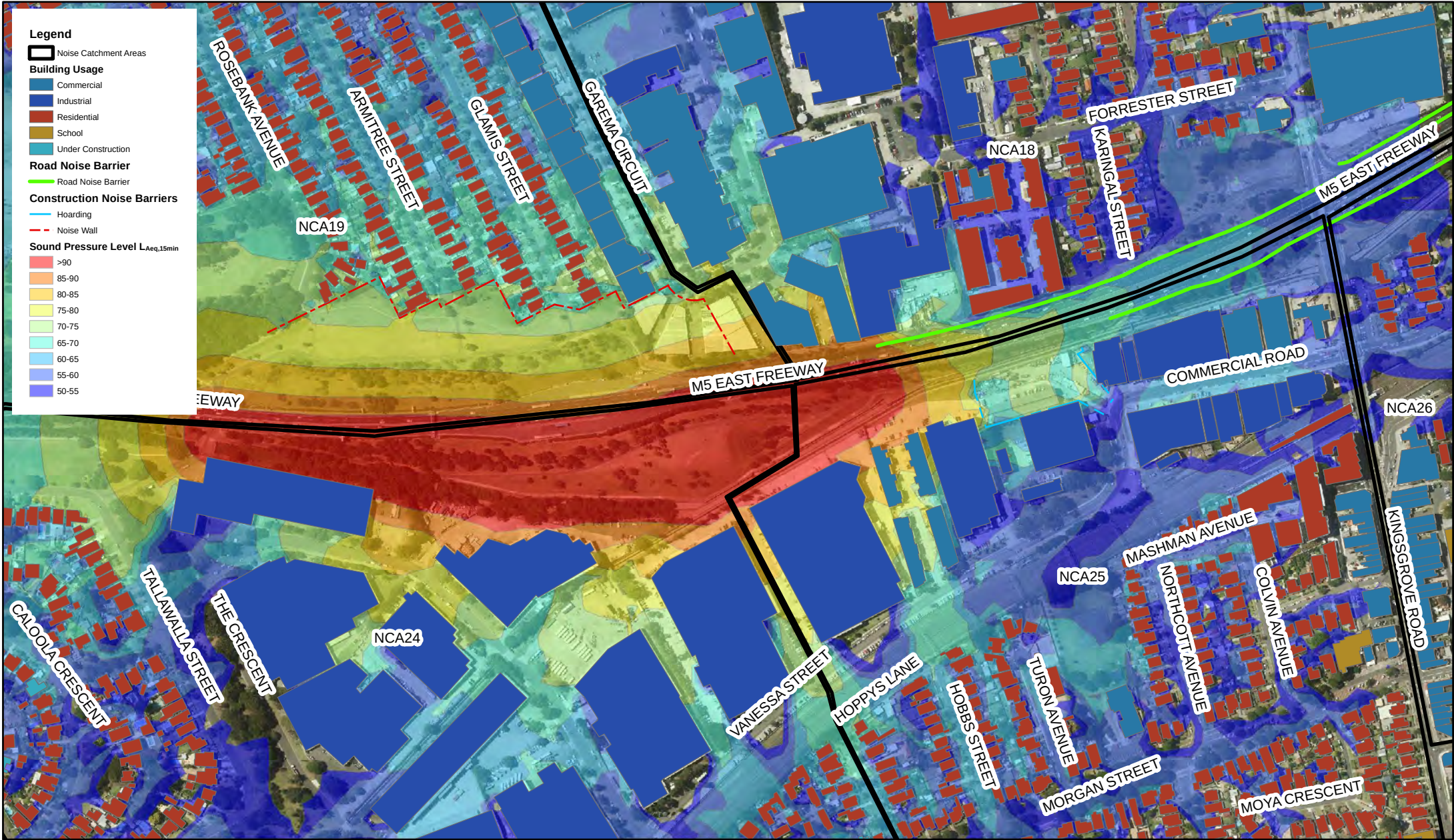
WestConnex Stage 2 - Construction Noise Assessment Surface works - Construction of ventilation stations - Workshop and deliveries - Day
