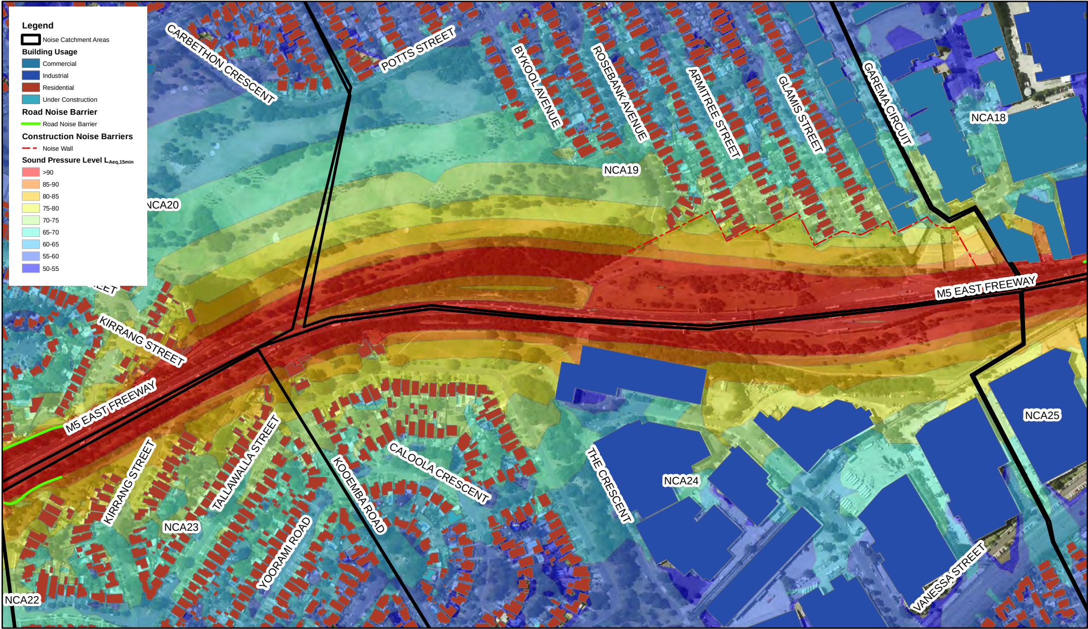
WestConnex Stage 2 - Construction Noise Assessment Surface works - M5 East Motorway road widening and realignment - Road tie-in works - Day
