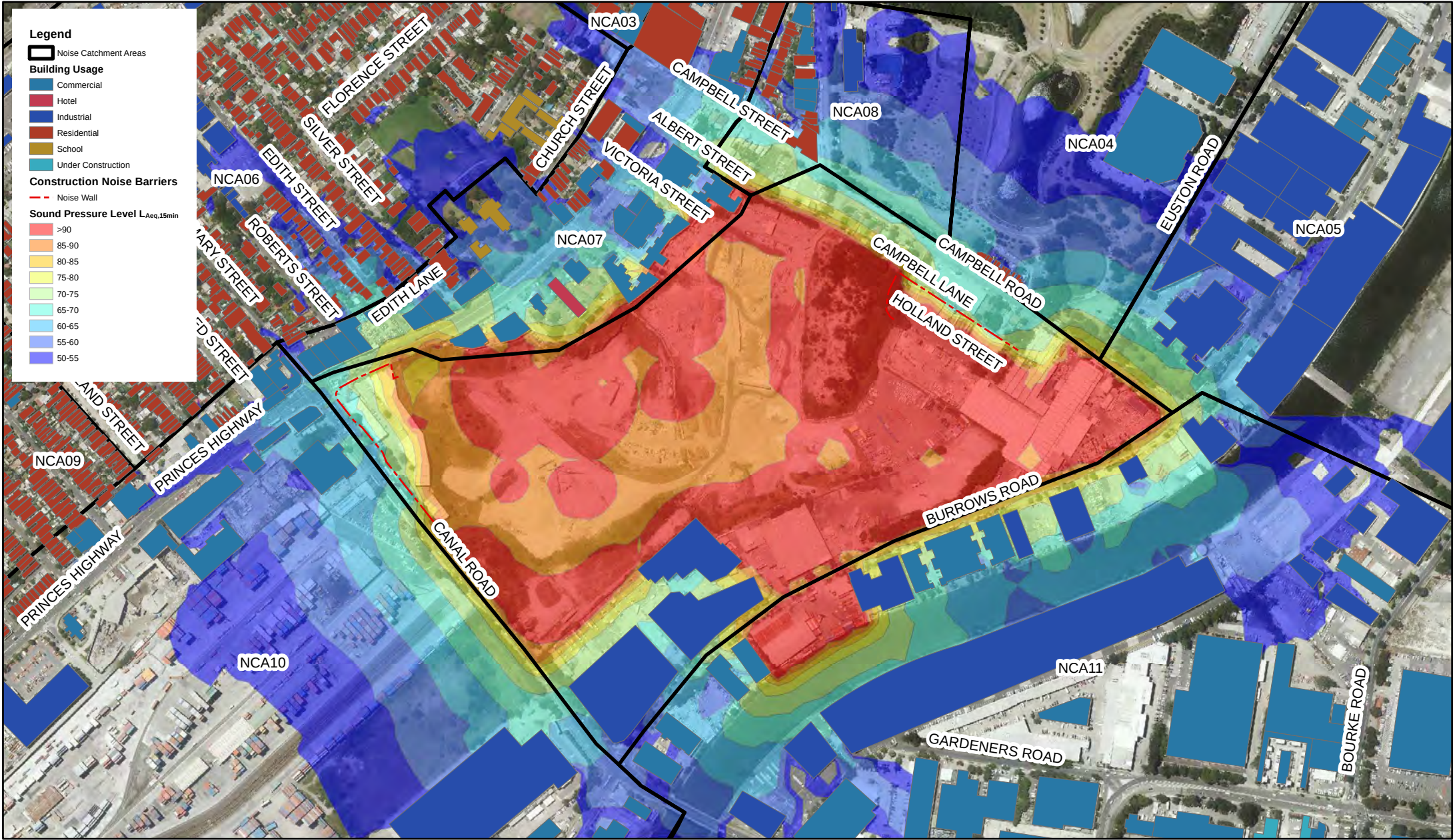
WestConnex Stage 2 - Construction Noise Assessment Surface works - Construction of SPI - Piling; ground improvement - Day
