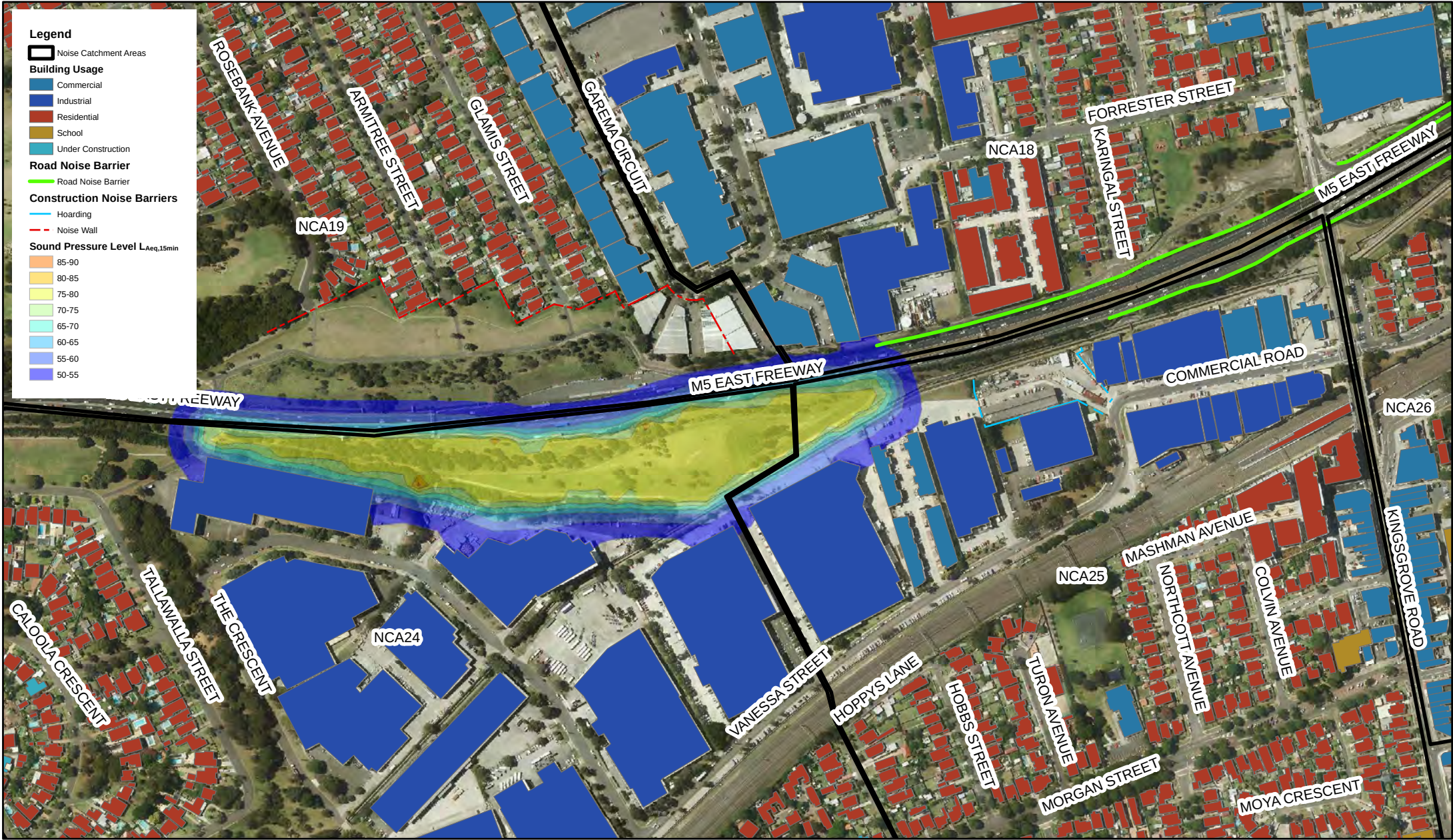
WestConnex Stage 2 - Construction Noise Assessment Surface works - Construction of ventilation stations - General worksite and car parking - Day
