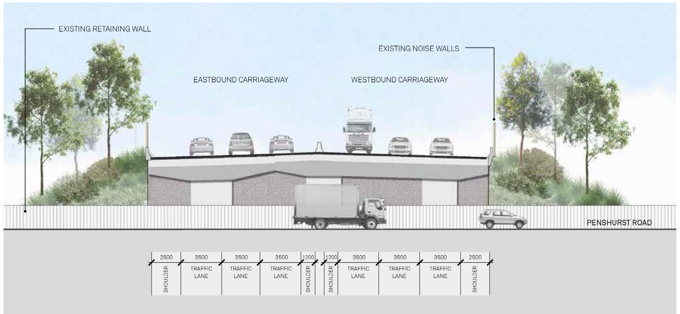
SECTION 1 / CH. 1500 (BRIDGE OVER PENSHURST ROAD) EXISTING
