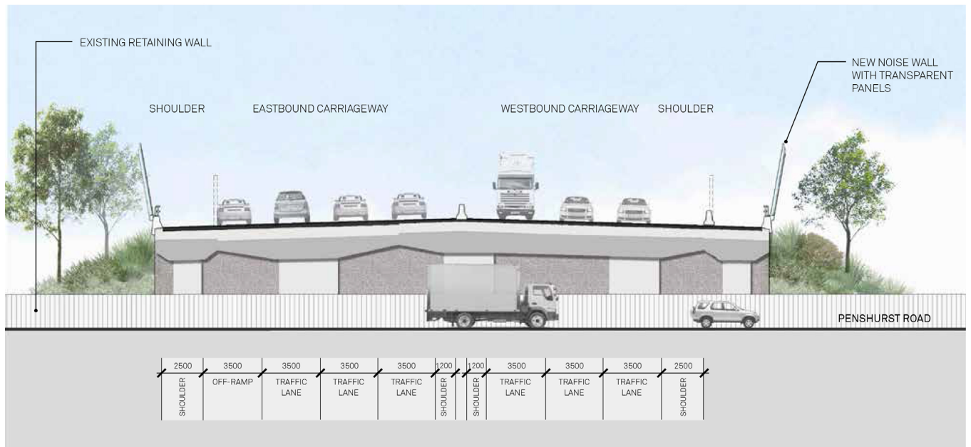
SECTION 1 / CH. 1500 (BRIDGE OVER PENSHURST ROAD) PROPOSED
