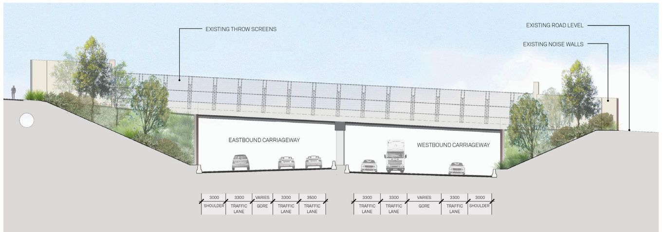
SECTION 2 / CH. 2300 (NEAR COOLOONGATTA ROAD BRIDGE) EXISTING
