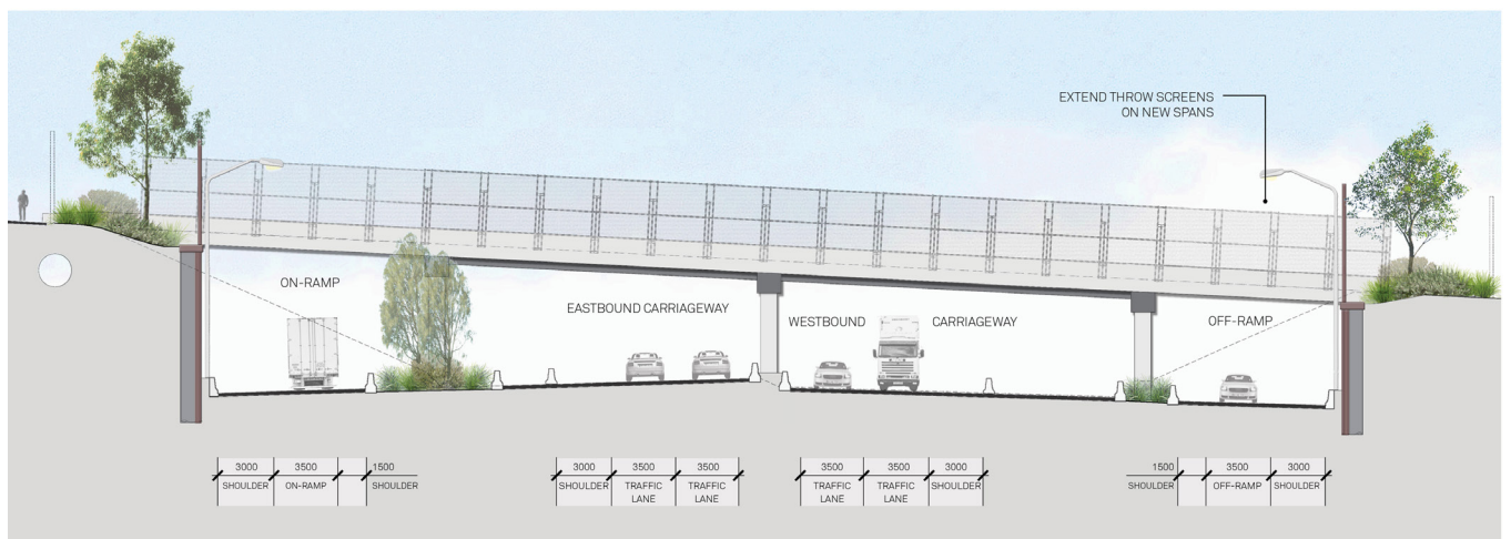
SECTION 2 / CH. 2300 (NEAR COOLOONGATTA ROAD BRIDGE) PROPOSED
