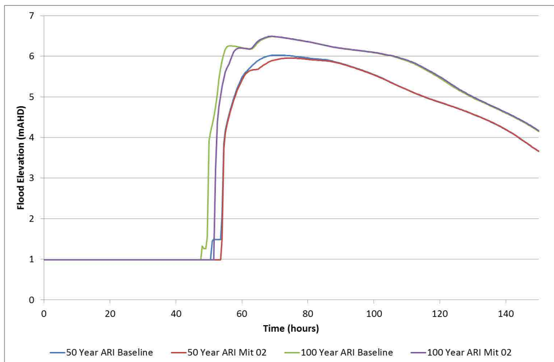
Figure 5-7 Alamy Creek (Fry St), North Grafton, design flood elevations, Option 2
