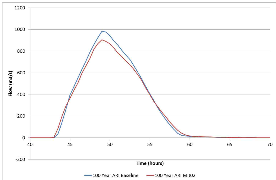
Figure 5-5 South Grafton levee overtopping flow, Option 2 (100 year ARI)
