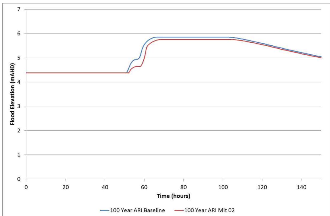
Figure 5-9 Iolanthe St, South Grafton, design flood elevations, Option 2 5
