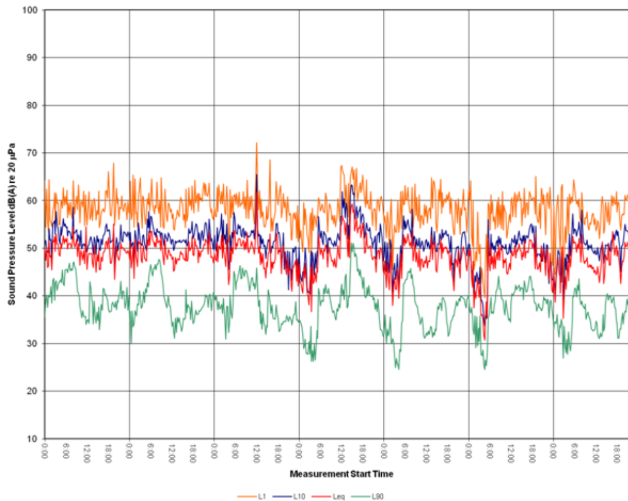
Figure 30: Measured Noise Levels – Logger Location 15 – Thursday 15 September to Wednesday 21 September 2011, dB re 20 µPa
