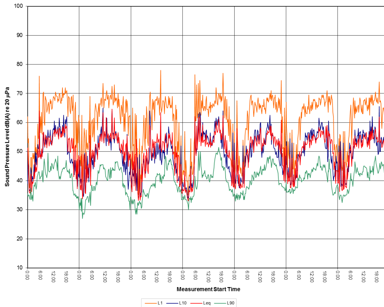
Figure 36: Measured Noise Levels – Logger Location 25 – Friday 18 October to Thursday 24 October 2013, dB re 20 µPa
