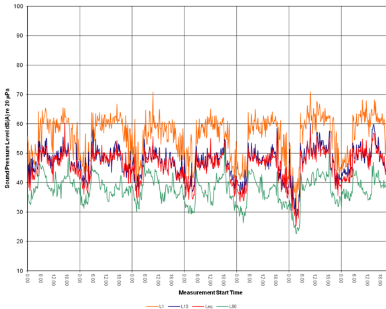
Figure 26: Measured Noise Levels – Logger Location 11 – Thursday 15 September to Wednesday 21 September 2011, dB re 20 \mu Pa
