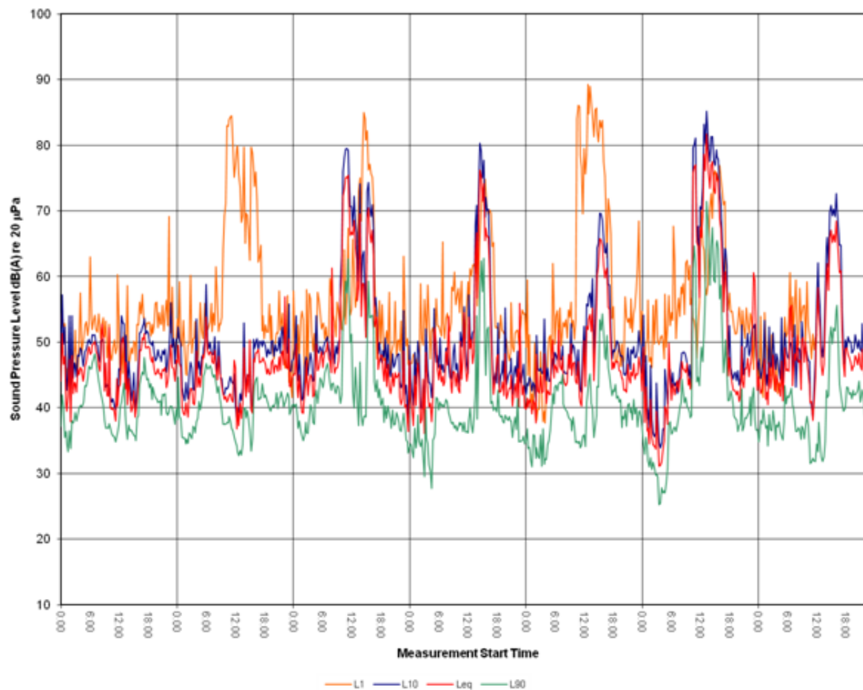
Figure 34: Measured Noise Levels – Logger Location 19 – Thursday 15 September to Wednesday 21 September 2011, dB re 20 µPa
