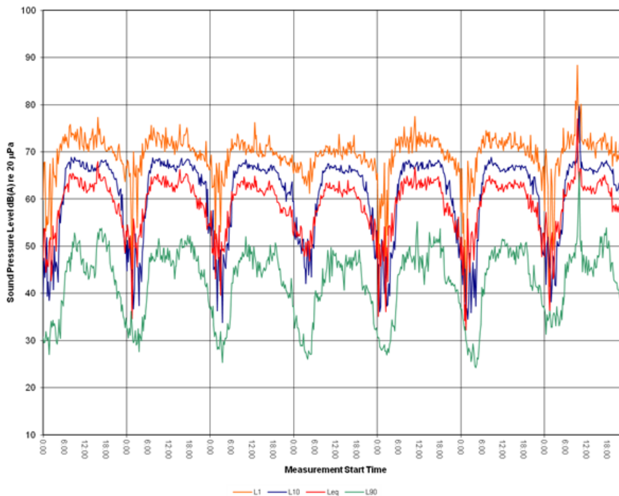
Figure 32: Measured Noise Levels – Logger Location 17 – Thursday 15 September to Wednesday 21 September 2011, dB re 20 µPa
