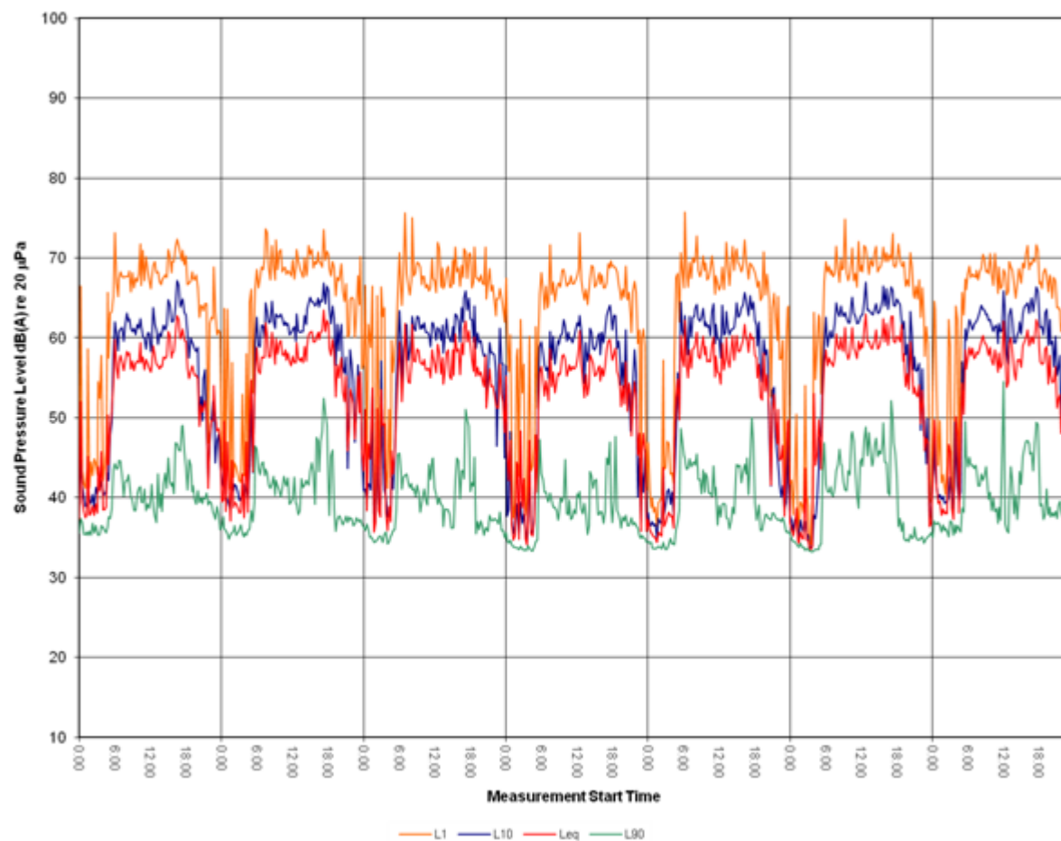
Figure 23: Measured Noise Levels – Logger Location 8 – Thursday 15 September to Wednesday 21 September 2011, dB re 20 µPa
