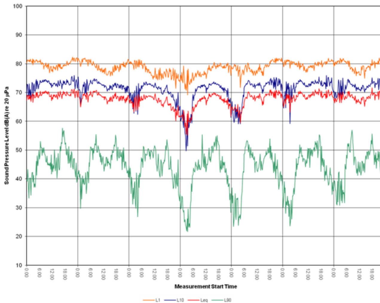
Figure 33: Measured Noise Levels – Logger Location 18 – Thursday 15 September to Wednesday 21 September 2011, dB re 20 µPa
