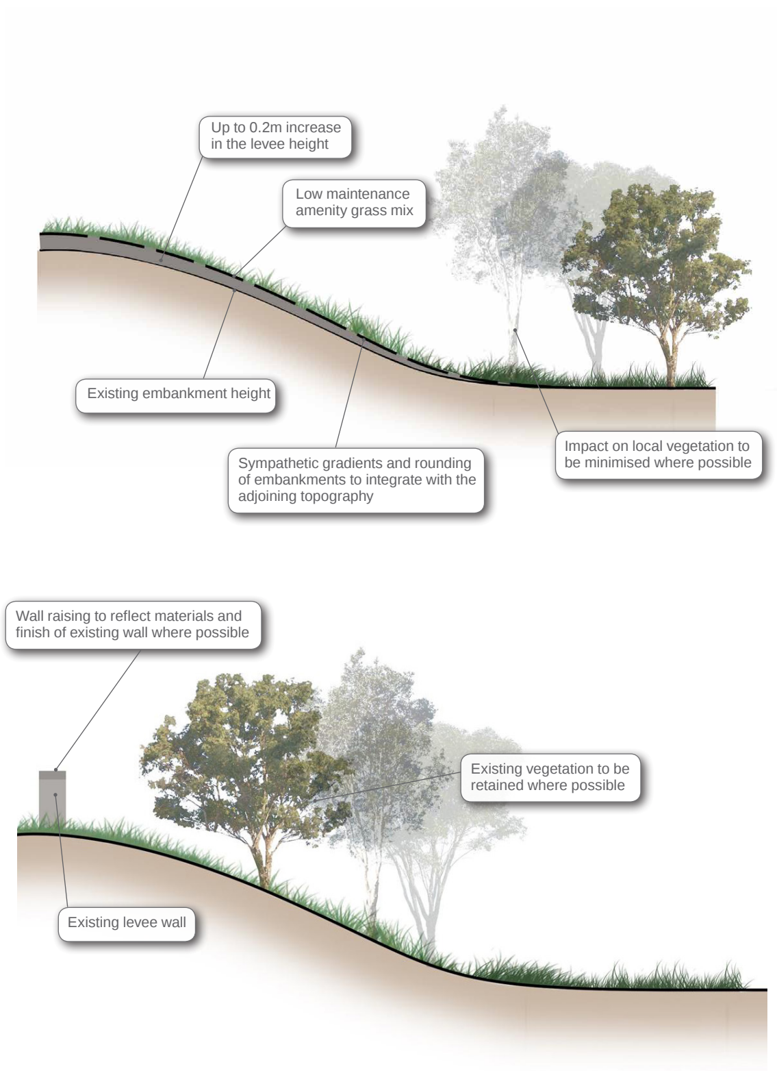
Landscape typical cross sections to inform detailed design stage
