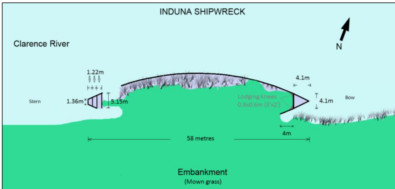
Plate 60: Site Plan of the SS Induna (FMW29) (Source: Comber Consultants)
