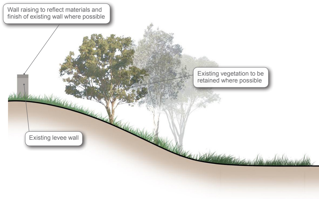
Landscape typical cross sections to inform detailed design stage
