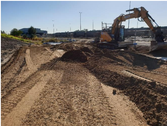
Figure 3: Leg 1 western drainage line culvert (19/06/20)
