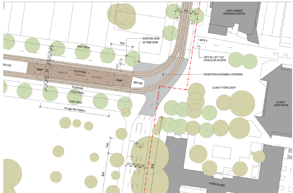
Figure 27 – UNSW High Street Stop - Plan
