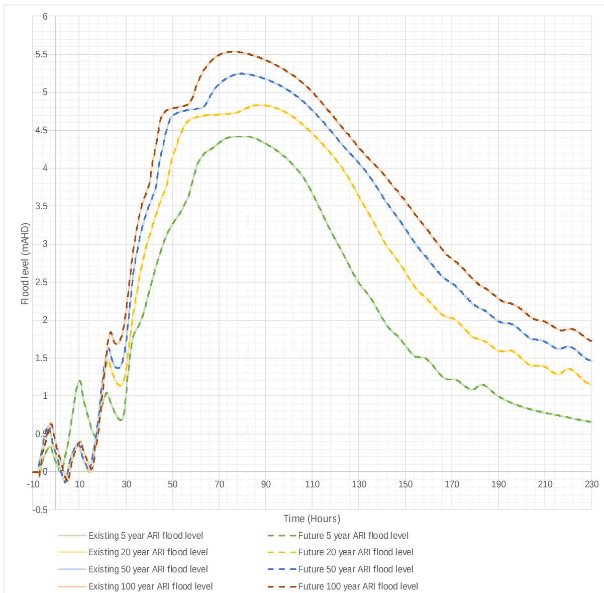
Figure 5.1 Flood level hydrographs at Richmond River at Bungawalbin Junction (CH130400)
